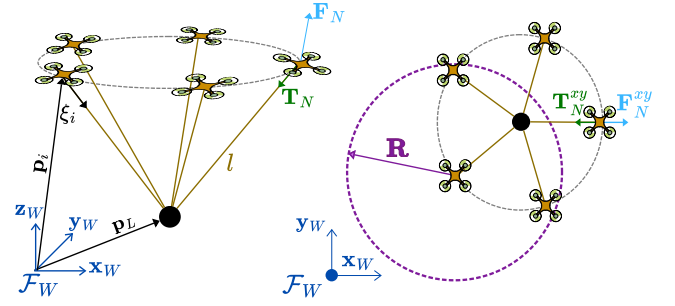
Figure 2: Overview of the cooperative load carrying system. Left: N UAVs cooperatively hover while suspending a point-mass load via taut cables of length l , where unit vectors \boldsymbol{\xi}_i and tensions \mathbf{T}_i are shown in the world frame \mathcal{F}_W . Right: each UAV senses the relative positions of neighbours within its sensing radius R .
