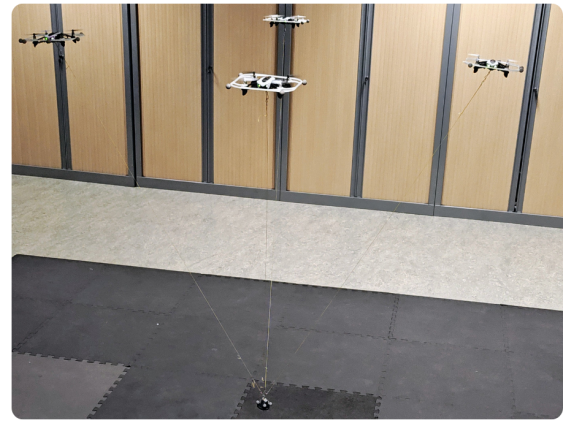
Figure 1: Experimental setup: four Parrot MAMBO mini-UAVs cooperatively carrying a cable-suspended load. A video of the experiments is available at youtu.be/fomDca2OPEA .
