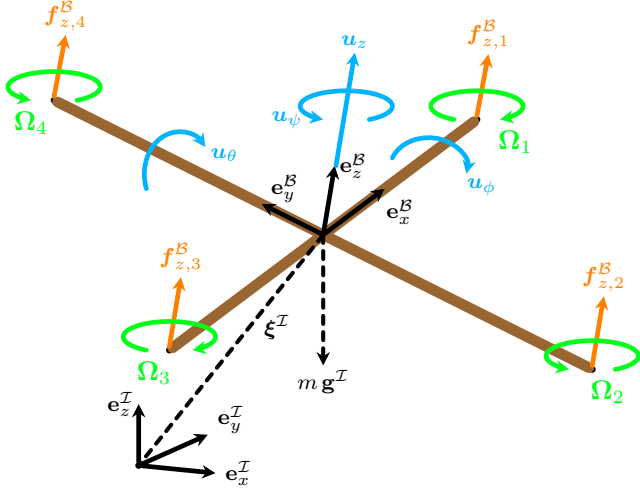
Figure 3: Free-body diagram of the quadrotor system model.
