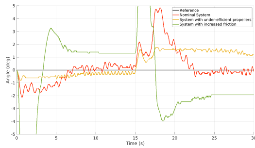
Figure 7: Yaw response, RMC, 10 blades nominal system
