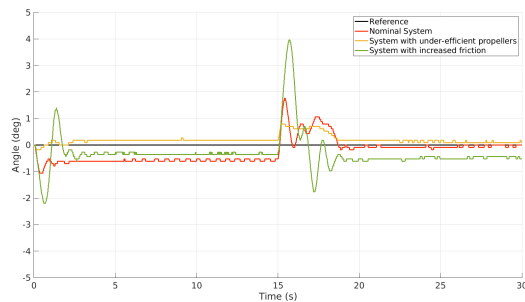
Figure 8: Yaw response, flatness controller, 10 blades nominal system
