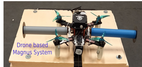
Figure 1: Magnus Effect-based Quadcopter prototype.
