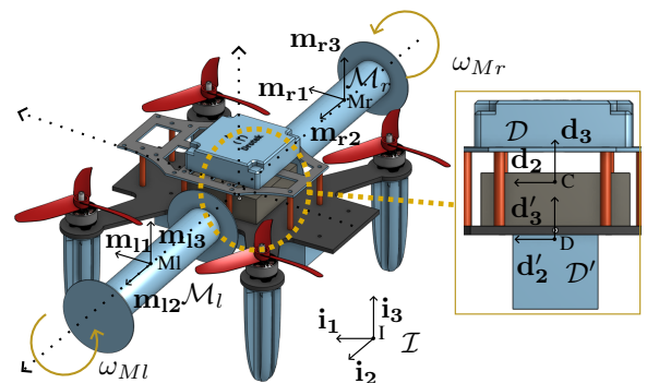
Figure 2: Frame definition on the quadcopter. From figure, \mathcal{D} represents the body frame, \mathcal{D}' the drone body frame, \mathcal{M}_l the left Magnus frame, \mathcal{M}_r the right Magnus frame and eventually \mathcal{I} the inertial frame.
