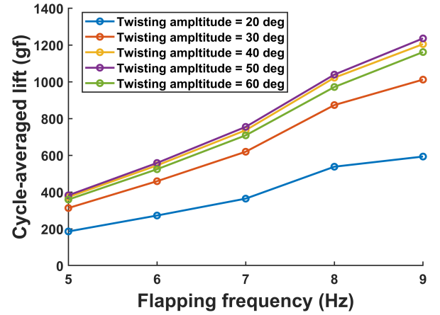
Figure 3: Cycle-averaged lift
