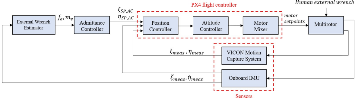
Figure 11: Experimental test system
