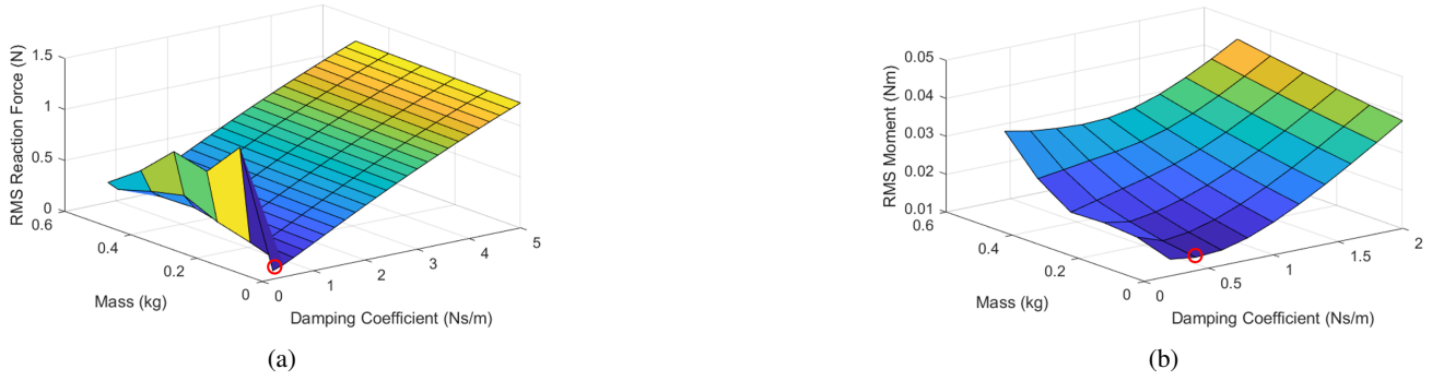
Figure 6: Parameter sweep of m_x and c_x values for (a) a 1m x -axis drag and m_\phi and c_\phi for (b) a 5deg roll-axis drag simulations to optimize for minimal RMS reaction force and moment, respectively, during interaction. Red circle indicates the optimal point for each of the parameter sweeps.
