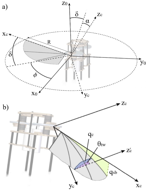
Figure 3: a) Illustration of wing kinematic parameters. Wing kinematics consist of three rotations, expressed with respect to a fixed coordinate system x_0y_0z_0 . The centre of x_0y_0z_0 corresponds to the wing centre of rotation. x_0 is parallel to the wing when it is at midstroke. x_0y_0 spans the body horizontal plane. x_cy_cz_c follows the wing motion. The stroke angle \phi is a rotation of the wing inside the body horizontal plane, around z_0 . The deviation angle \delta is a rotation around the rotated y-axis. Deviation is the wing out-of-plane motion. The inclination angle \alpha is a rotation around the x_c -axis. The inclination angle determines the angle of incidence. At zero inclination angle, the wing surface is parallel to z_0 . R is the single wing span, measured along the leading edge from the wing centre of rotation to the wing tip. b) Illustration of wing deformation parameters. x_cz_c corresponds to the rigid wing plane. Spanwise bending is defined as the leading edge deformation perpendicular to the wing plane, along y_c . The twist angle \theta_{tw} is the angle between x_cz_c and a chord line that connects the local leading edge and trailing edge. Camber q_c is the distance to the local wing chord, measured perpendicular to the chord line going from leading edge to trailing edge.
