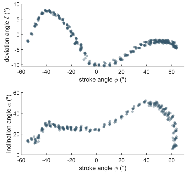
Figure 4: Evolution of a) deviation angle and b) inclination angle throughout stroke. The wing moves from left to right.
