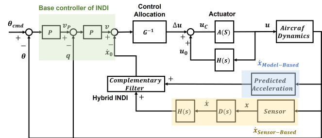
Figure 3: Control structure of the hybrid INDI control
