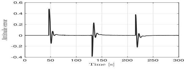
Figure 4: Attitude error (P_a(\tilde{R}_\psi))^v .
