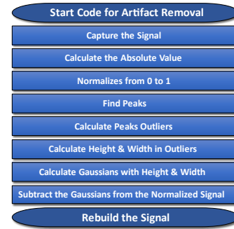
Figure 4: Proposed algorithm for automatic removal of artifacts in real-time.
