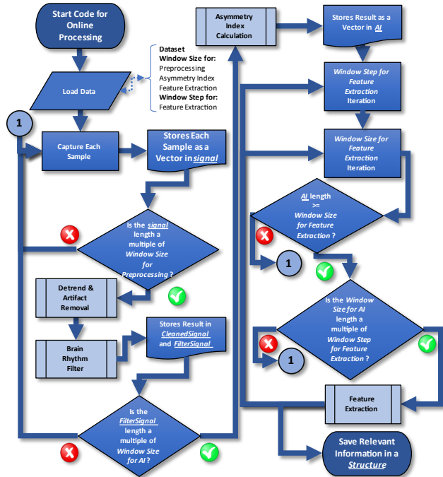
Figure 3: Flowchart proposed for real-time signal processing.
