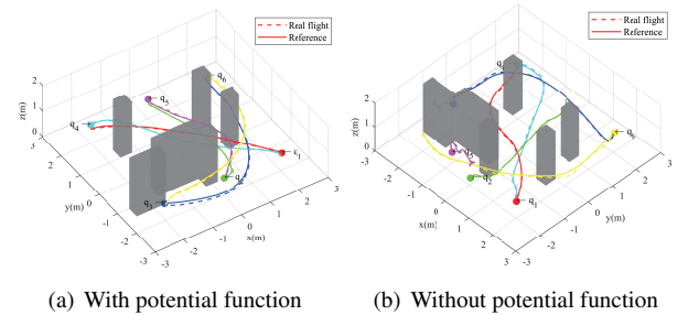
Figure 6: The 3D navigation of multi-quadrotors in cluttered environments with non-convex obstacles.
