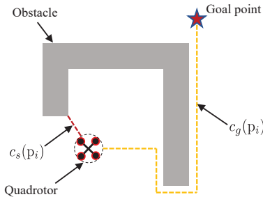
Figure 4: The illustration of deadloack avoidance.
