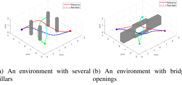
Figure 5: Quadrotor trajectories during antipodal position swapping. In both (a) and (b), the solid circles denote four quadrotors and the solid curves denotes their trajectories, respectively.
