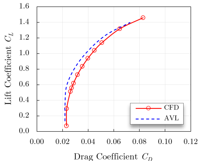
Figure 10: Polar.
