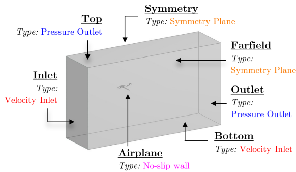
Figure 4: Boundary conditions.
