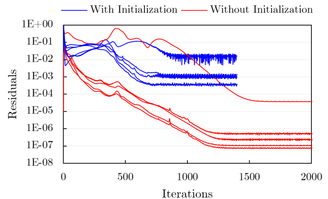
Figure 5: Residuals.
