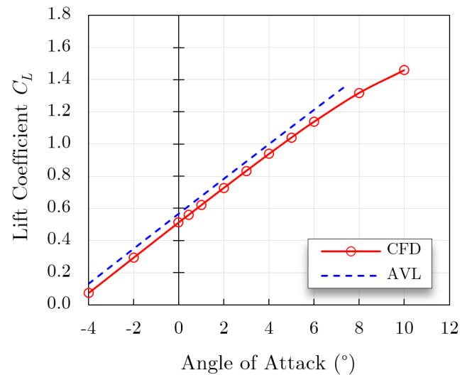
Figure 9: Lift curve.
