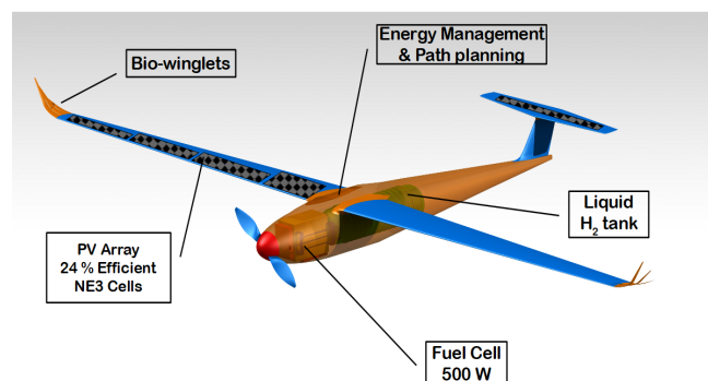
Figure 1: Drone Mermoz v1 - 12 kg and 3.6 m span demonstrator of technology.
