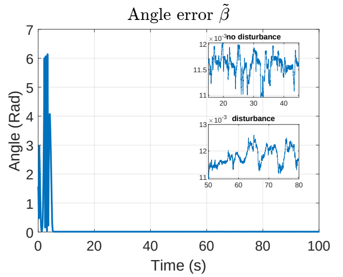
Figure 7: Error angle \tilde{\beta} .
