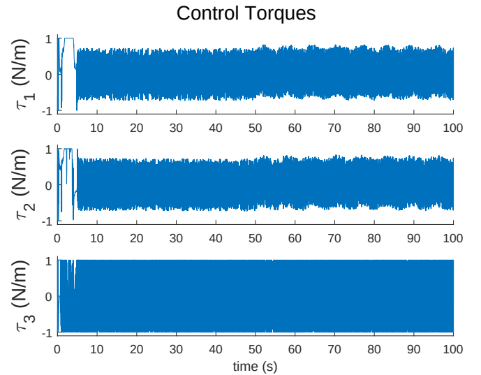
Figure 8: Control torques.
