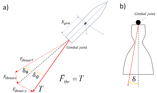
Figure 1: a) Aircraft with an integrated TVC mechanism, b) Gimbal mechanism: A gimbal is essentially a universal joint.
