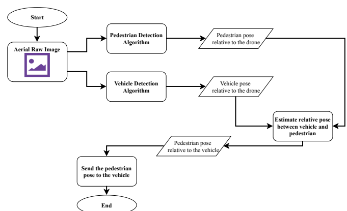
Figure 1: Proposed Approach
