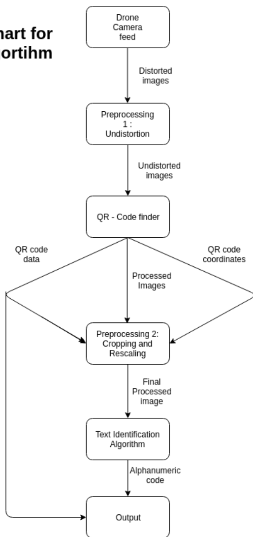
Figure 2: Flowchart for the algorithm
