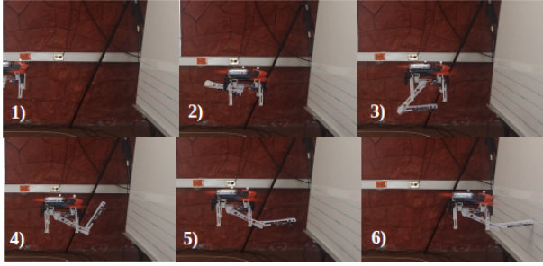
Figure 9: Sequence of successful contact of the aerial manipulator with the rigid surface.
