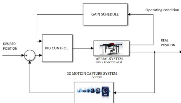
Figure 5: Block diagram of the proposed system with GS-PID control [1].
