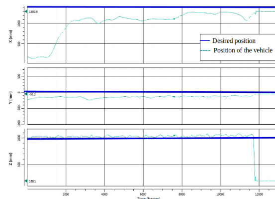
Figure 7: Behavior of the aerial vehicle carrying the robotic arm with standard PID control.
