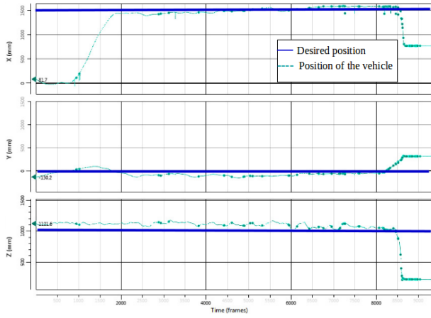
Figure 8: Behavior of the aerial vehicle with the robotic arm extended near to rigid surface, GS-PID control
