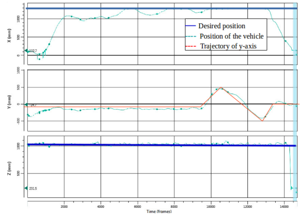
Figure 10: Behavior of the aerial manipulator in full contact with the rigid surface, GS-PID control.
