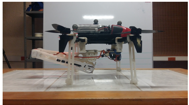
Figure 3: Aerial manipulator, physical implementation.
