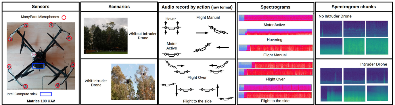
Figure 2: General overview to record the audio in two different environments and generate a dataset.
