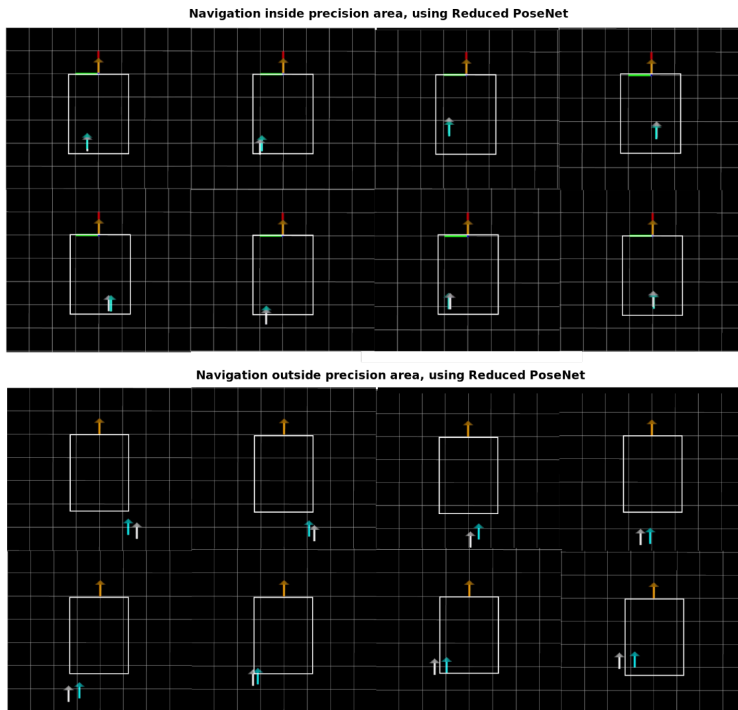
Figure 9: Predicted pose compared with groundtruth using RVIZ. First row shows Groundtruth (white) and Predicted (Sky) comparison results by Reduced PoseNet inside the precision area. Second row shows comparison results by Reduced PoseNet outside precision area.
