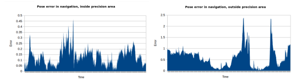
Figure 8: Error over time in navigation. Left graph shows the error while navigating inside the precision area. Right graph shows the error while navigating outside the precision area.
