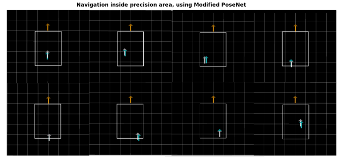
Figure 6: Predicted pose compared with groundtruth using RVIZ. White arrow shows Groundtruth and Blue arrow Predicted.
