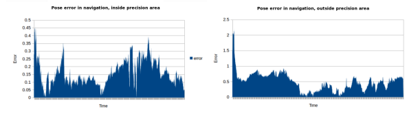
Figure 7: Error over time in navigation. Left graph shows the error while navigating inside the precision area. Right graph shows the error while navigating outside the precision area.
