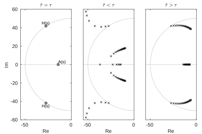
Figure 4: Effect of uncertainty in actuator delay on significant poles of INDI loop (sample time T_s = 0.001 sec), \tau/T_s = 40, 0 < \hat{\tau}/T_s < 80
