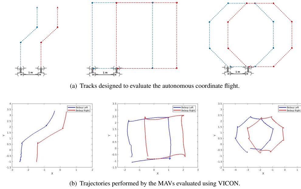
Figure 4: Tracks predefined to perform coordinate flight, the blue line represent the left MAV trajectory and the red line correspond to the right MAV.
