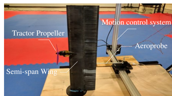
Figure 3: Test set-up in ENAC indoor flight arena
