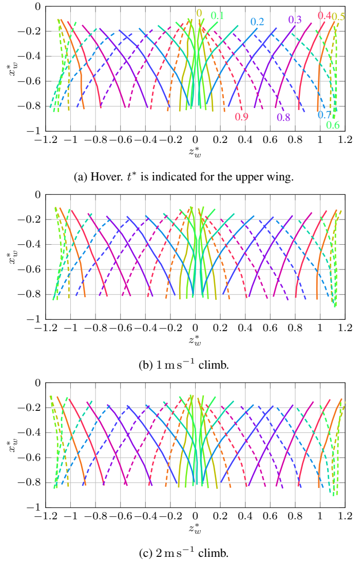
Figure 5: Wing profile deformation at s_w = 100 \text{ mm} over the flapping cycle due to different climbing velocities. The upper wing can be seen in the right half, the outstroke profiles are dashed.
