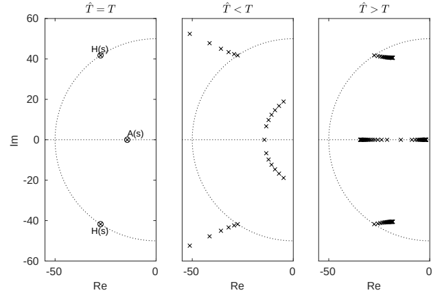
Figure 3: Effect of uncertainty in actuator dynamics on significant poles of INDI loop, T = 0.07, 0.01 < \hat{T} < 0.14
