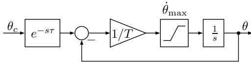
Figure 7: Actuator Model
