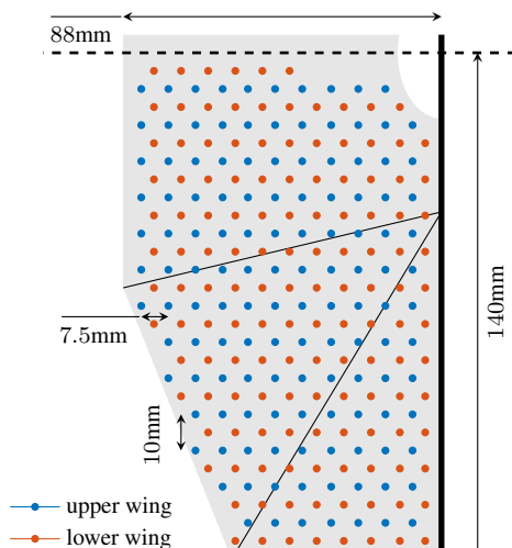
Figure 3: Schematic of DelFly wing half with point grids.
