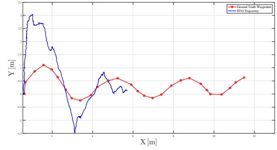
Figure 3: The trajectory of camera vs. the ground thruth path
