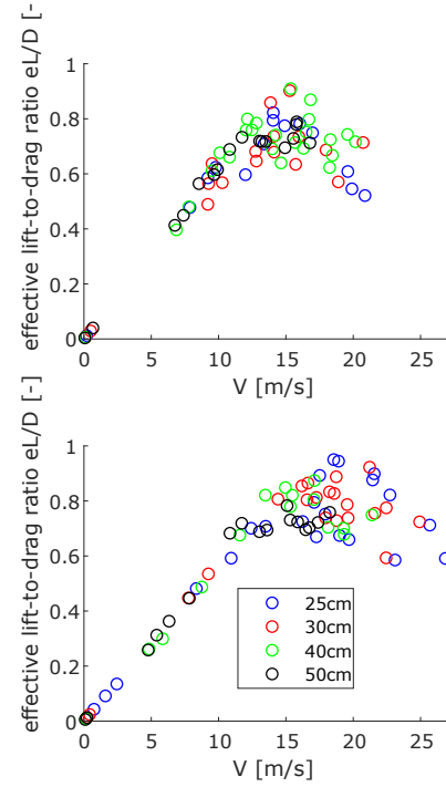
Fig. 9: Calculated effective lift-to-drag ratio at pitch angles from hover to -45^\circ for four different body diameters and two total masses. Top: 2.13kg . Bottom: 2.50kg .
