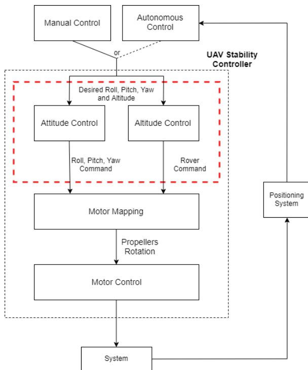
Figure 2: Overall Control Block Diagram
