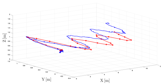
Figure 5: 3D trajectory of camera vs. the ground truth path
