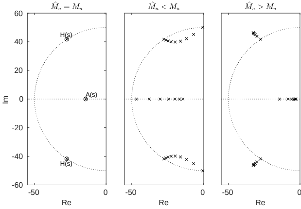
Figure 2: Effect of uncertainty in control effectivity on significant poles of INDI loop, 0.2 < \hat{M}_u/M_u < 4
