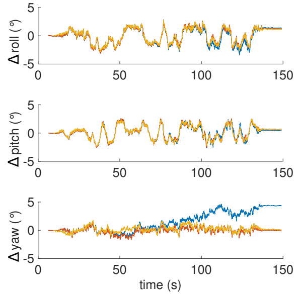
Figure 6: Roll, pitch and yaw error for a single run with simulated sun vector measurements. Blue: without polarization compass, red: with polarization compass using static projection, yellow: with polarization compass using dynamic projection.
