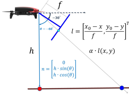
Figure 3: Geometric configuration used to generate a synthetic depth image to be used by ORB-SLAM in its RGB-D version, to obtain a pose estimation with metric. Image taken from [19].
