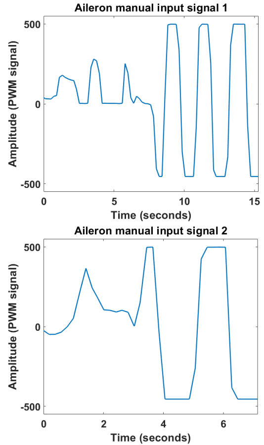
Figure 4: Realizations of arbitrary aileron manual input signals.
