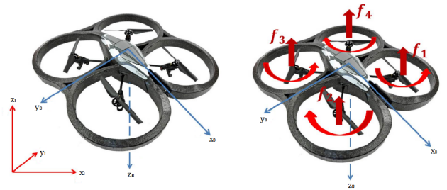
Figure 3: Inertial and Body frames
