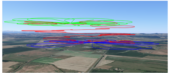
Figure 11: Simulation of 3 UAVs sampling 2 horizontal planes and the last one covering the outer 3D border.
