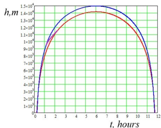
Figure 10: Altitude as function of time for the airplane and conditions investigated. Blue line — low atmosphere model (9), red line — isothermal model (10), purple — interpolation between the models.
