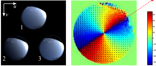
Figure 3: Estimation of sun position from the three images of the polarization sensor. Left: The camera image containing the three sub-images after de-bayering. In this example the sun is located outside the field of view of the camera. A bright cloud visible in the upper right corner of the sub-images indicates the approximate sun direction. Intensity differences between the three sub-images allow to estimate polarization degree and angle for each pixel. For example, quite strong intensity differences can be observed in the lower left corner of the three sub-images indicating high degree of polarization. Right: Shown are the sky polarization angles, i.e. the angles of the polarization vectors with respect to the local meridians (great circles of constant azimuth) in color code, ranging from -90^\circ (blue) to +90^\circ (red), and polarization vectors \mathbf{f}_i with length scaled according to weight w_i (black arrows), projected onto the image plane. The red cross in the upper right corners depicts the estimated position of the sun (approx. -34.5^\circ azimuth and +36^\circ elevation angle with respect to the camera frame).
