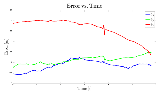
Figure 11: The XY errors of the quadrotor center with the moving platform center with 1.5\text{m/s} velocity with sliding controller
