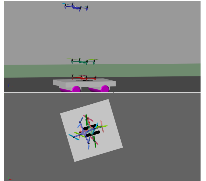
Figure 1: Comparison among virtual drones with three controllers in MATLAB Simscape dynamic space. The red drone refers to PID, the green one to SLD, and blue drone to MRAC controller.
