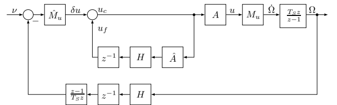
Figure 1: Controller structure
