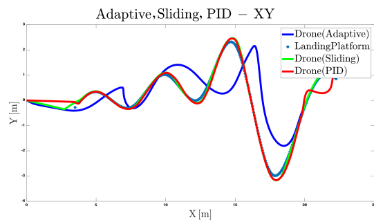
Figure 7: The XY comparison of three controllers to the landing platform with 2.5\text{m/s} velocity in MATLAB Simscape
