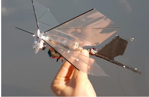
Figure 1: DelFly II MAV. The used model omits the tail and electronics. [11]
