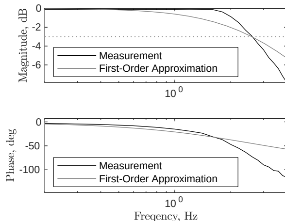
Figure 10: Bode plot of servo dynamics
