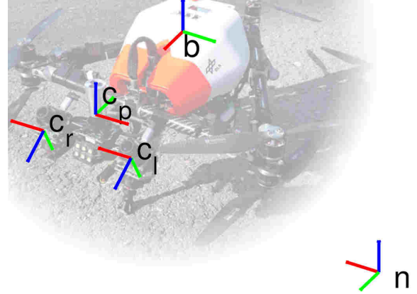
Figure 4: An image of ARDEA with the navigation frame (n-frame), the body frame (b-frame), the frames of one stereo pair ( c_1 - and c_r -frame) and the frame of the camera with the polarization compass (p-frame).
