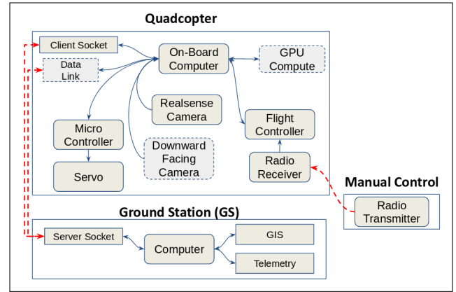
Figure 2: Overview of sub systems and how they are connected. Red links represent wireless communication. Grey dashed boxes are specific to the outdoor vehicle only.
