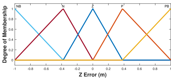
Figure 8: Input Membership Function - Z Error
