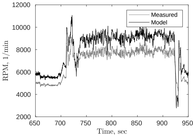
Figure 8: BLDC/ESC model
