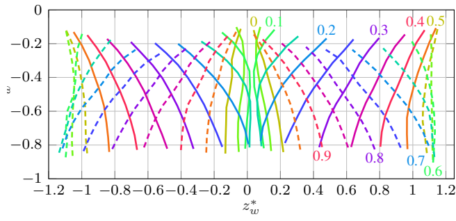
(a) 0.5 \text{ m s}^{-1} forward flight at \theta_b = 70^\circ . t^* is indicated for the upper wing.
