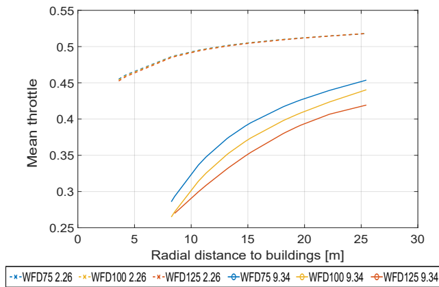
Figure 11: Mean throttle value respect to the radial distance to the buildings for six different atmospheric conditions: WFD i for i = 75, 100, 125 is the wind field with the Dryden noise, i being the percentage of W20 used for the simulation. Dashed lines represent the data for W20 = 2.26 \text{ m/s} and solid lines, W20 = 9.34 \text{ m/s} .
