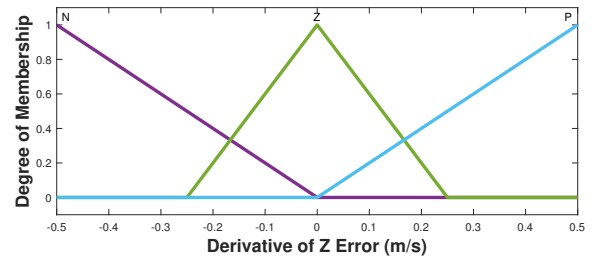
Figure 9: Input Membership Function - Derivative of Z Error
