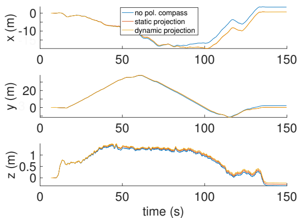
Figure 7: Estimated position of ARDEA during an outdoor experiment with and without the polarization compass.
