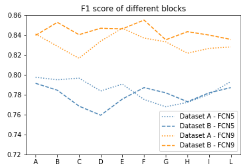
Figure 2: F1 performance of FCN5 and FCN9 across different blocks of images, which differ only in the scene illumination.
