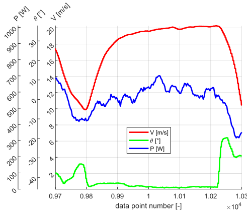
Fig. 4: Illustration of one run out of the recorded data during a flight. The multicopter accelerates to a steady-state velocity of 20\text{m/s} for a constant pitch angle of -45^\circ .
