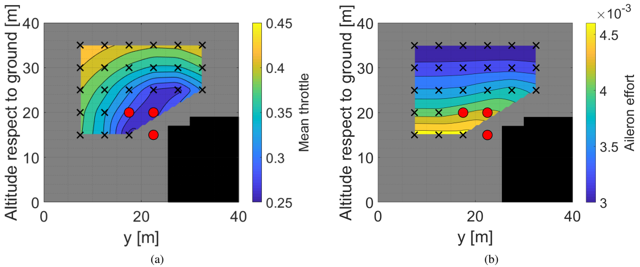
Figure 13: Contour plot of the mean throttle command and the CE of the aileron for W_{20} = 9.34 m/s. The colour maps are based on the interpolation of the successful flights. The red circles represent the flights that crashed against the ground or the buildings during simulation.
