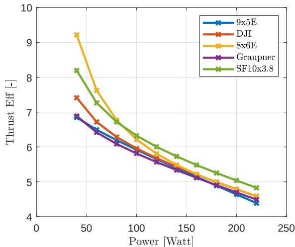
Figure 4: Thrust efficiency in function of power for a selected combination of propellers.
