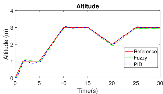
Figure 17: Altitude Control
