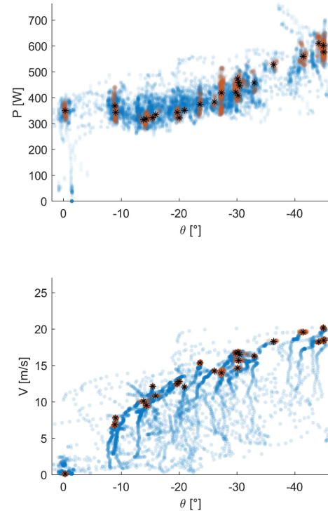
Fig. 5: Total power consumption and horizontal velocity as a function of the pitch angle for the configuration with 2.13\text{kg} and 40\text{cm} . Blue: all recorded data during the test flight. Orange: recorded data during identified steady-state regime. Black: average values for each steady-state regime
