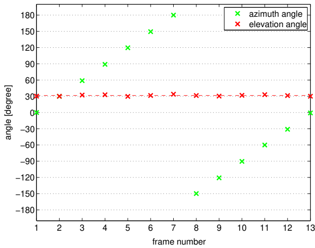
Figure 5: Test of the sun position estimation by turning the multicopter in 30^\circ steps. Shown are the azimuth angle with respect to the initial orientation (green 'x') and the sun elevation angles (red 'x') as estimated by the polarization compass. The dashed line shows the true sun elevation angle ( \approx 32^\circ ).
