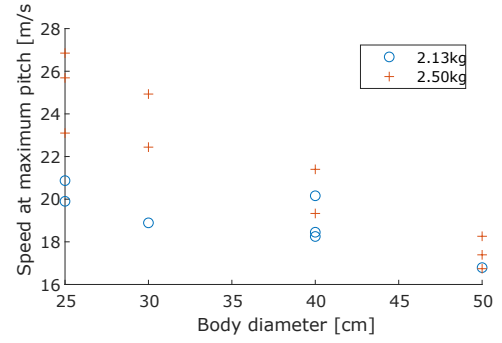
Fig. 7: Measured top speeds at -45^\circ as a function of the body diameter for two masses.
