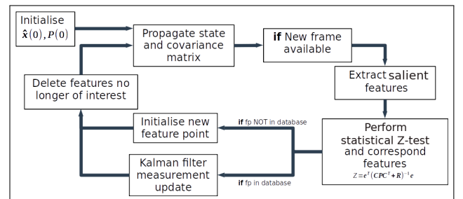
Figure 4: The feature point (fp) tracking EKF process. N.B: this flowchart is invariant of the image processing method.
