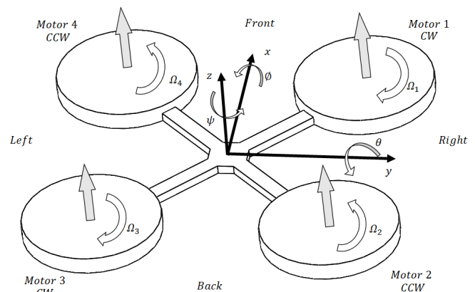
Figure 1: Quadcopter Representation
