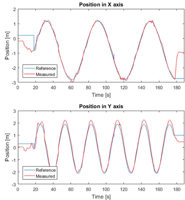
Figure 8: Gerono trajectory for an hexarotor with a failure in rotor 3.
