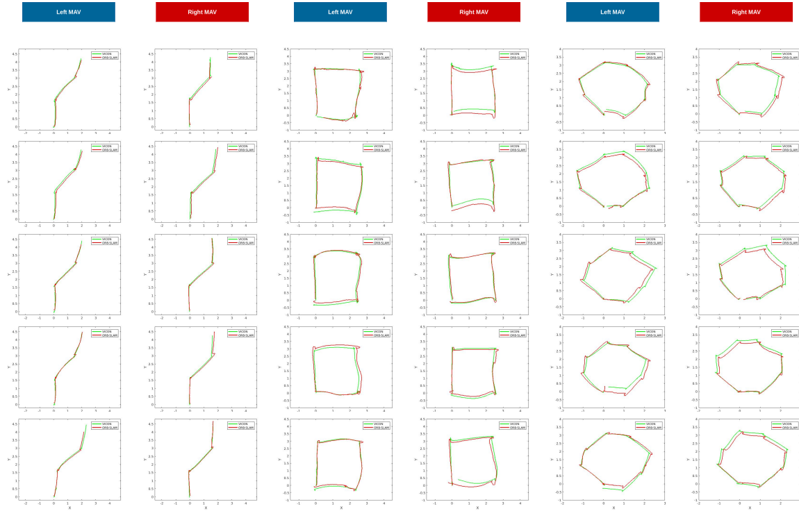
Figure 6: Examples of the trajectories generated. The green line represents the ground truth (VICON), and the red line is the path travelled by the vehicle. First, the graph of the vehicle placed on the left is shown, depending on the vehicle placed on the right.
