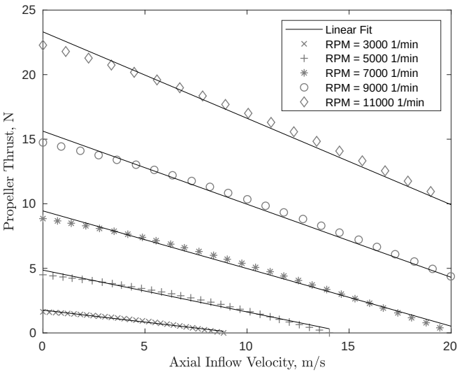
Figure 6: Thrust over axial velocity
