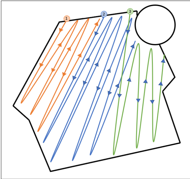
Figure 7: Predetermined path of each outdoor quadrotor.
