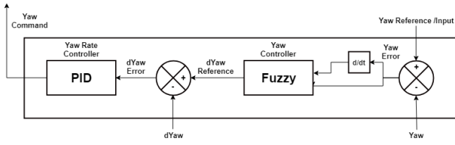
Figure 7: Nested Fuzzy-PID for Yaw Control
