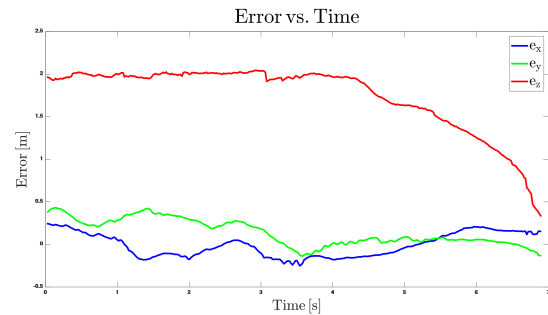
Figure 9: The XY errors of the quadrotor center with the moving platform center in with 0.5\text{m/s} velocity with sliding controller
