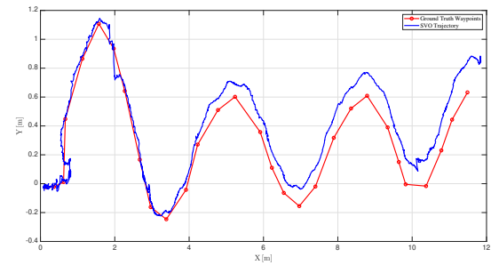
Figure 4: The trajectory of camera + IMU vs. the ground thruth path
