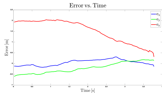
Figure 10: The XY errors of the quadrotor center with the moving platform center with 1.5\text{m/s} velocity with PID controller
