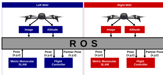
Figure 5: The architecture of the processing of our approach using ROS as a communication channel. Each PID controllers know the metric position of the partner to compensate the differences of the current pose to the reference point, this allows the flight are coordinate.
