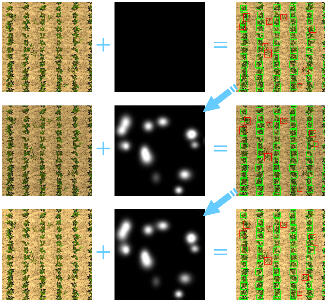
Figure 3: Classification over multiple passages. Each row correspond to a single passage over the same portion of the field, but with different illumination conditions (first column). The RGB image is coupled with a probability map derived from previous passages, when available (second column). The combined input provides an improved object detection across passages (third column). In the second passage, a weed is discovered in the center-right part of the image, but one in the bottom right is lost. In the third passage, the latter weed is detected again, and an additional weed is discovered among the first crop row on the left.
