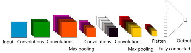
Figure 4: Architecture of the CNN. The input is a moving time window over the spectrogram, Mel spectrogram or MFCC. The output a binary value indicating whether aircraft sound is present or not.
