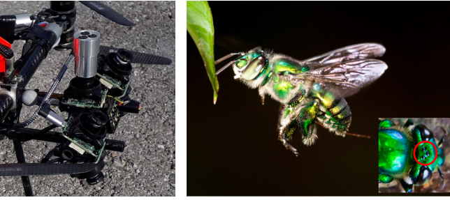
Figure 2: The polarization sensor, a standard camera with cylindrical polarizer unit mounted in front of the camera lens is positioned between the two stereo camera pairs (left). The sensor was inspired by the ocelli of orchid bees. As highlighted by the red circle in the inset of the right figure (shown is a close up view of the head of the bee Euglossa imperialis ), bees have three simple eyes with polarization sensitive photoreceptors (photos courtesy of Emily Baird, Stockholm University). In orchid bees, the preferred polarization orientation is very similar within each eye but differs between eyes by somewhat less than 60^\circ [3].
