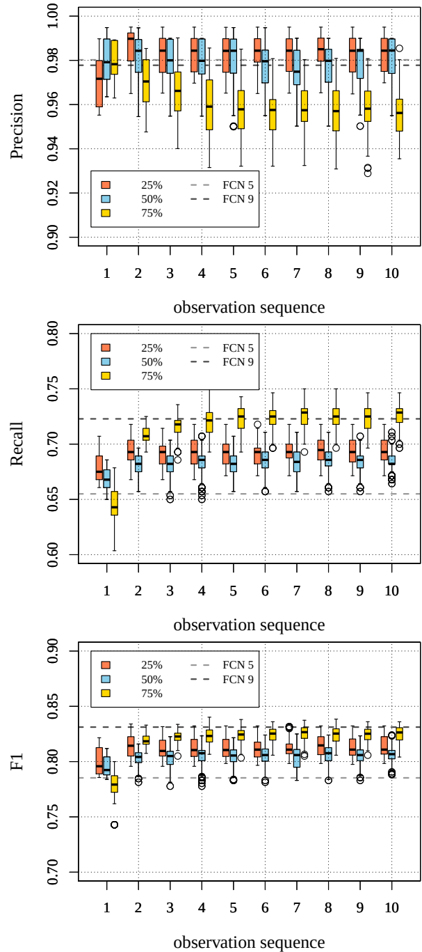
Figure 4: Precision, recall and F1-score on dataset A. The performance achieved with different training strategies (i.e., 25%, 50%, and 75% probability of having a probability map as input) is compared against the average performance of the FCN5 and FCN9 networks using only the RGB inputs.
