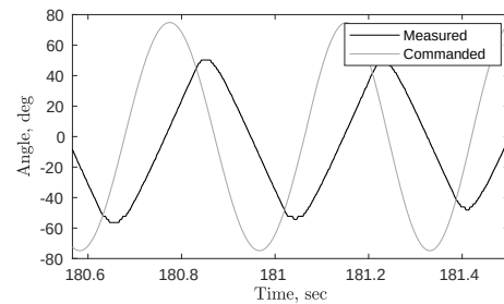
Figure 9: Servo dynamics at high frequencies
