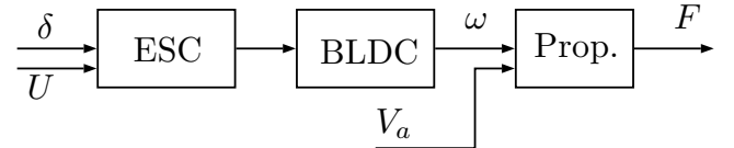
Figure 5: Motor model
