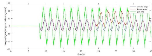
Figure 6 – flapping experiment
