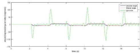
Figure 5 – non-flapping experiment
