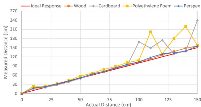
Figure 9: Infrared experimental response with electric motors on, for different target materials
