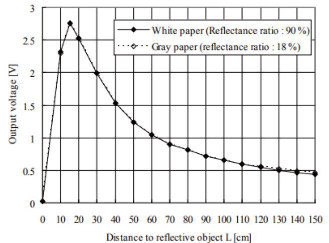
Figure 1: Output of the sensor vs. the distance.
