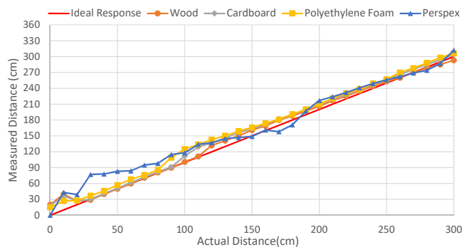
Figure 4: LiDAR experimental response with electric motors off, for different target materials
