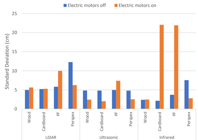
Figure 11: Standard deviation of the measurements.
