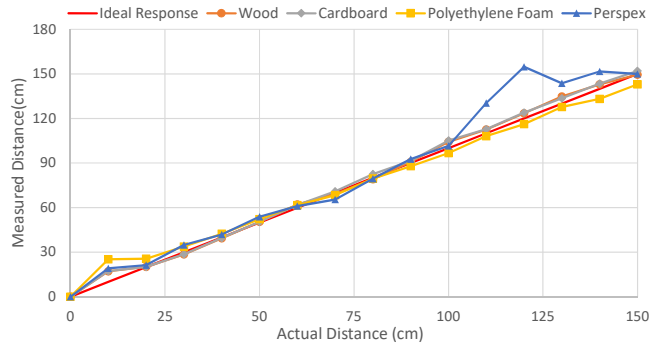
Figure 8: Infrared experimental response with electric motors off, for different target materials
