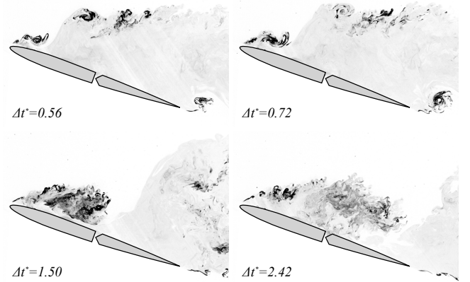
Figure 7: \alpha_{LE} = 20^\circ , \delta = 20^\circ \rightarrow 19^\circ , 6Hz
