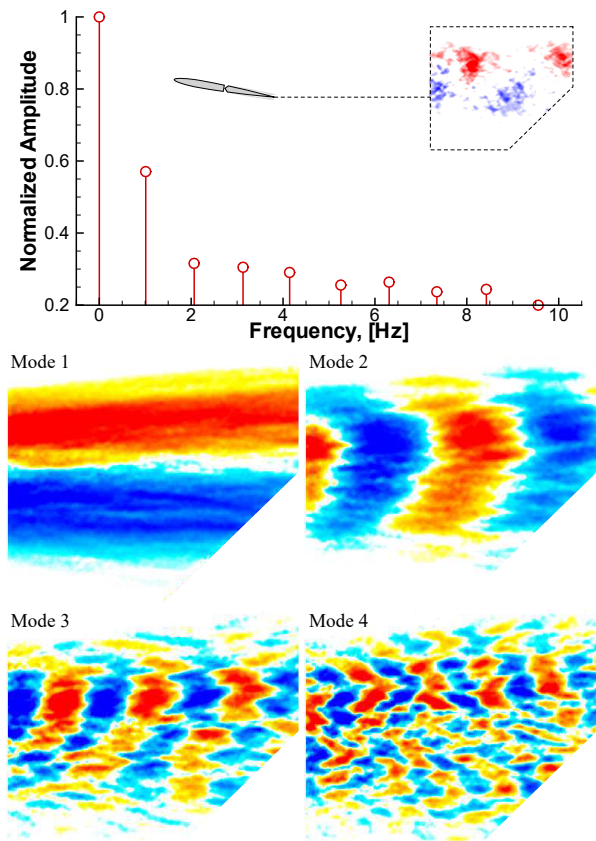
Figure 13: DMD of the near-body vorticity field: (top) normalized mode amplitude, (bottom) select modes.
