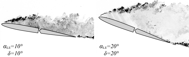
Figure 2: Baseline flow fields of static airfoils: (left) \alpha_{LE} = 10^\circ separated flow, (right) \alpha_{LE} = 20^\circ massively separated flow.
