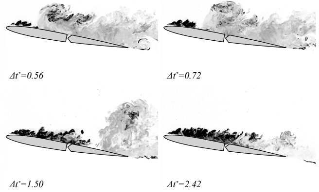
Figure 9: \alpha_{LE} = 10^\circ , \delta = 10^\circ \rightarrow 9^\circ , 6Hz
