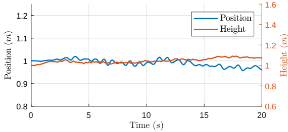
Figure 3: The position and height for scale = 1 in simulation
