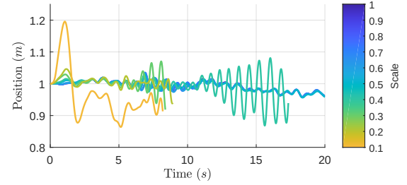
(a) The position of the quadrotor for different scales
