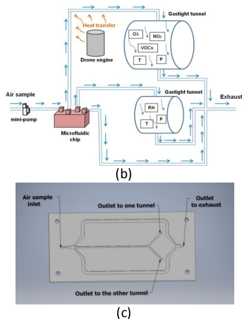
Figure 2 - Schematic representation of the microfluidic system for sampling during flight (a) and stationary sampling (b); Proposed design of the microfluidic chip for flow restriction inside the system (c)
