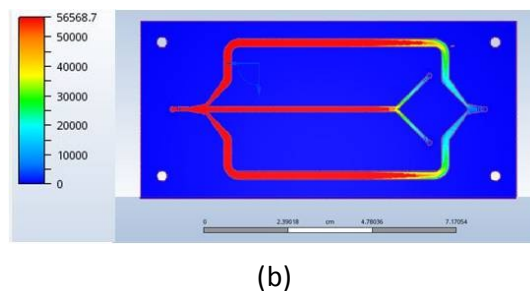
Figure 3 - Flow simulations on the microfluidic chip: Flow division between external and central microchannel (a); flow division between the two tunnels (b). The scale represents the velocity amplitude.
