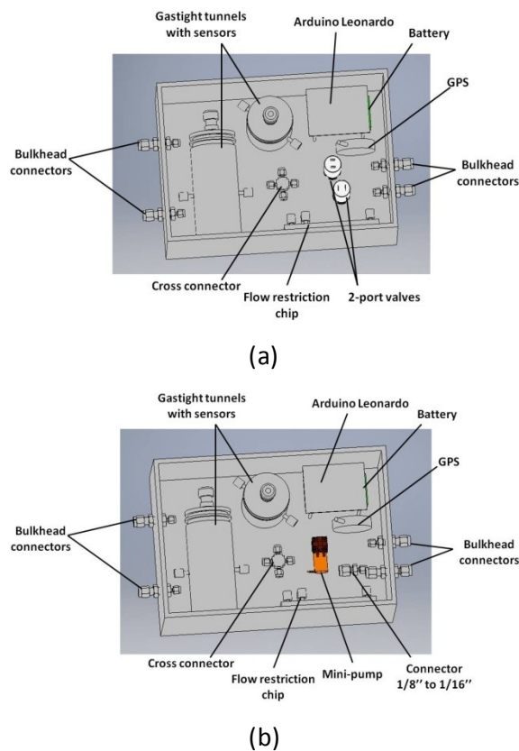
Figure 4 - 3D design of the total monitoring system for sampling during flight (a) and stationary sampling (b).
