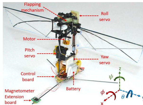
Figure 1 - KUBeetle
