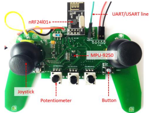
Figure 3 – Remote control
