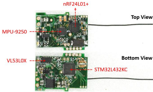
Figure 2 - Control board
