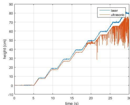
Figure 7 – Altitude estimation
