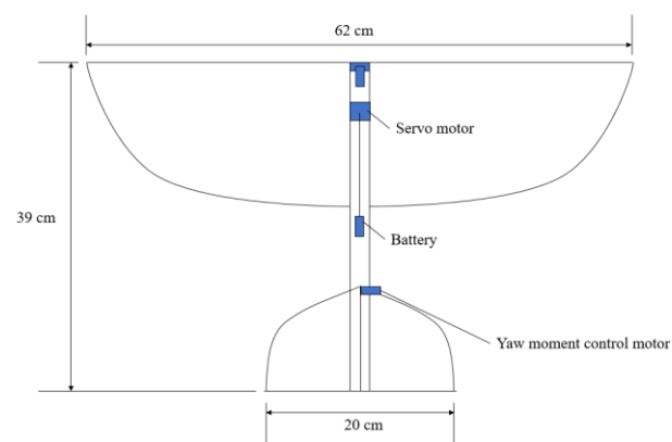
Figure 2 – Dimensional outline of WiFly and components arrangement
