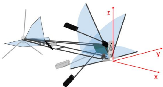
Figure 4 - Definition of internal axes of WiFly
