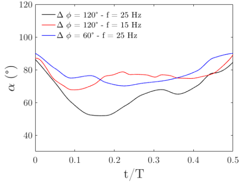
Figure 9: Comparison of instantaneous angles of attack extracted from HSV for cases with \Delta\phi = 120^\circ , frequency f = 25\text{Hz} ; \Delta\phi = 120^\circ , frequency f = 15\text{Hz} and \Delta\phi = 60^\circ , frequency f = 25\text{Hz} .
