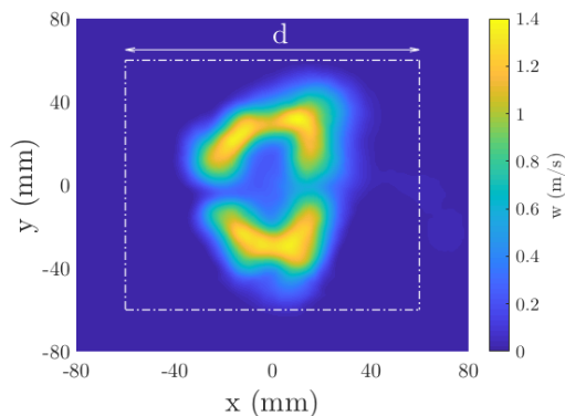
Figure 3: Contours of vertical velocity obtained from PIV measurements for wings operated at a frequency of 25 Hz and with an amplitude of 120°.
