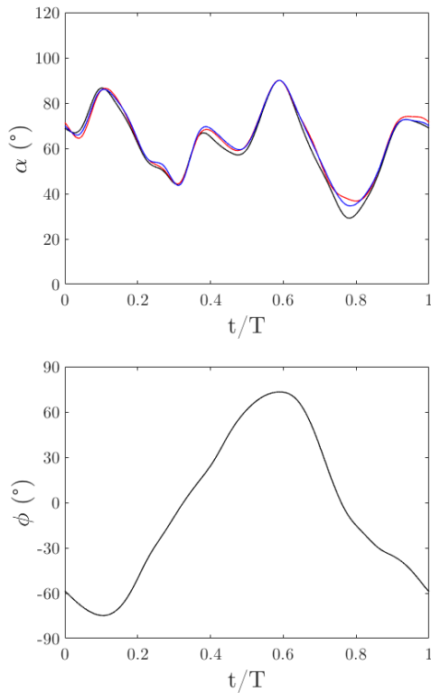
Figure 6: Instantaneous angle of attack and effective flapping angle as a function of non-dimensional time, extracted from HSV for flapping amplitude \Delta\phi = 120^\circ and frequency f = 25\text{Hz} . \alpha is shown for three consecutive flapping cycles.
