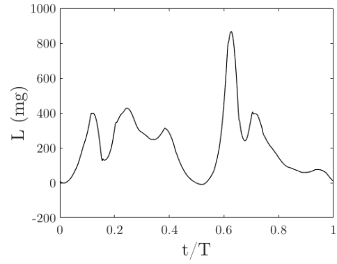
Figure 10: Instantaneous lift obtained numerically for wings operated with flapping amplitude \Delta\phi = 120^\circ and frequency f = 25\text{Hz} .
