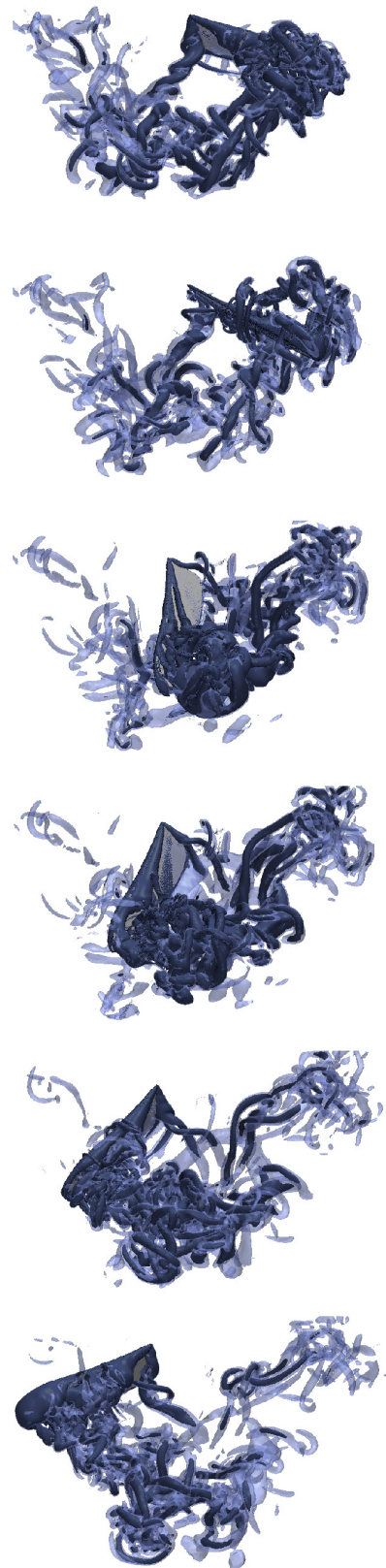
Figure 11: Sequence of Q-criterion isosurfaces obtained from DNS for flapping amplitude \Delta\phi = 120^\circ and frequency f = 25\text{Hz} .
