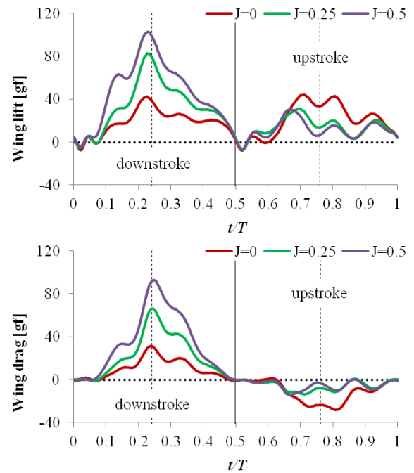
Figure 7 - Time-course lift and drag for various J s
