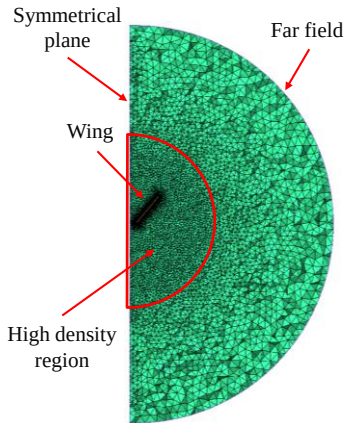
Figure 4 - A cross section of the volume mesh
