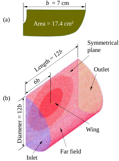
Figure 3 - (a) Wing geometry. (b) Computational domain
