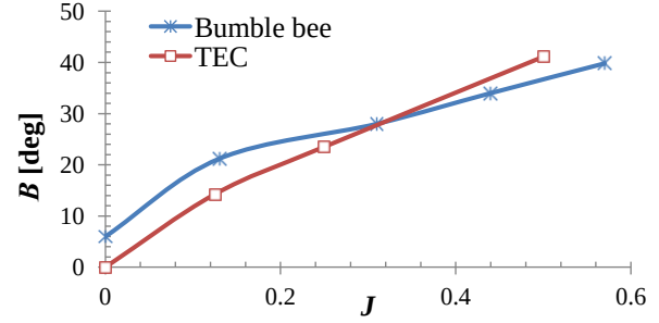
Figure 9 - Stroke plane angle for equilibrium during forward flight
