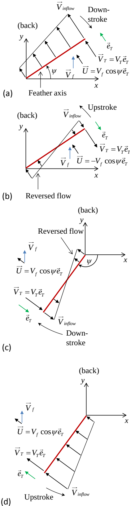
Figure 6 - Inflow in KU-Beetle. (a) During downstroke, -90^\circ < \psi < 90^\circ . (b) During upstroke, -90^\circ < \psi < 90^\circ . (c) During downstroke, \psi < -90^\circ or \psi > 90^\circ . (d) During upstroke, \psi < -90^\circ or \psi > 90^\circ .
