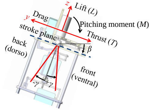
Figure 1 - Control variable, the red lines indicate the wing root
