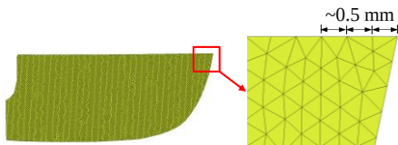
Figure 5 - Mesh on the wing surface
