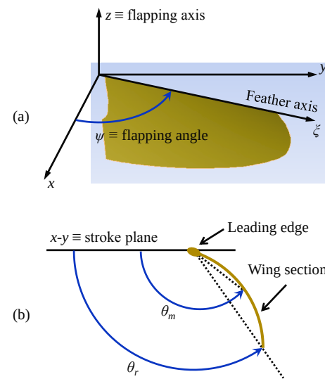
Figure 2 - Wing motion. (a) Three-dimensional wing motion. (b) Wing camber
