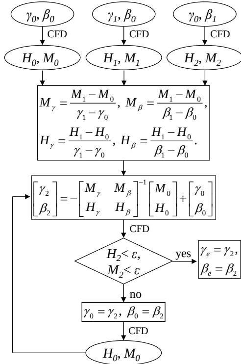
Figure 8 - Flow chart for acquiring equilibrium
