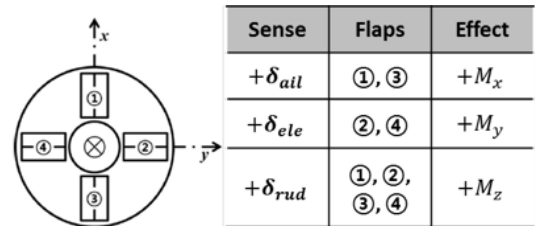
Figure 1: control flaps sign conventions.
