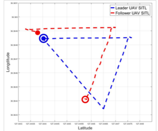
Figure 9: In the simulation 2D path.
