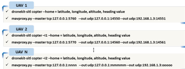
Figure 6: Connect dronekit-sitl and MAVProxy.
