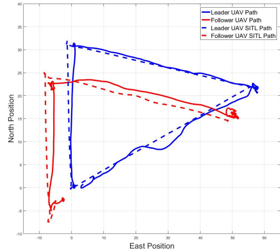
Figure 13: 2D path (Formation Flight Test).
