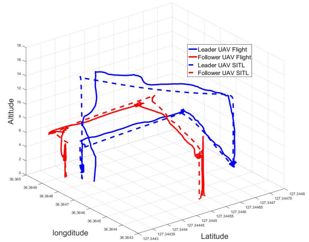
Figure 14: 3D path (Formation Flight Test).
