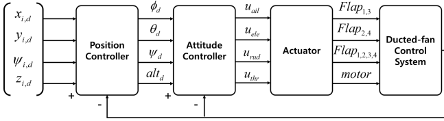
Figure 3: Ducted-fan UAV's control system diagram.
