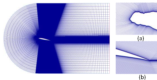
Figure 2 – 0° IM Aerofoil mesh at 14.5° AoA, with detail (a) leading-edge (b) trailing-edge
