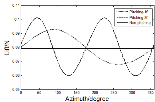
(a) Lift.
