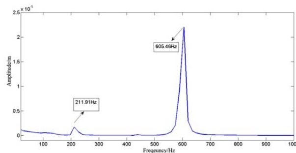
Figure 11 – Amplitude spectrum of displacement
