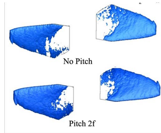
Figure 7 – Iso-surface of vorticity for the non-pitch nano rotor and the pitching nano rotor.
