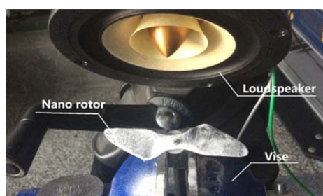
Figure 2 - Modal test bench for nano rotor.
