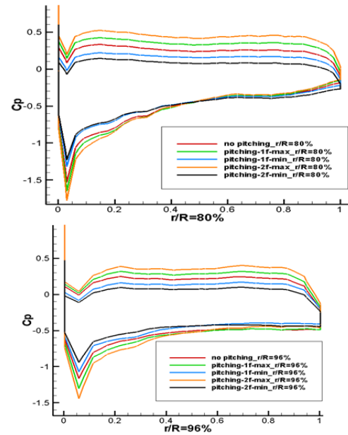
Figure 6 - Pressure coefficient comparison at different blade sections for different cases.
