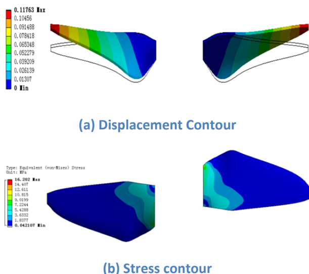
Figure 10 - Displacement and stress contour of the nano rotor.
