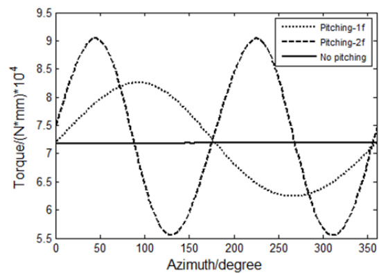
(b) Torque
