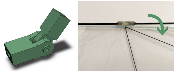
Figure 2: CAD model of the hinge (left), the hinge placed on the leading edge of the wing (right).
