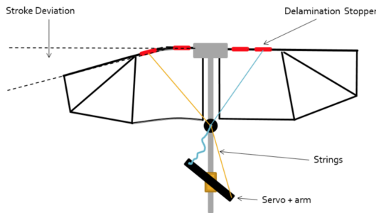
Figure 4: Bending of the leading edge using servo and string based actuation mechanism from the front view.
