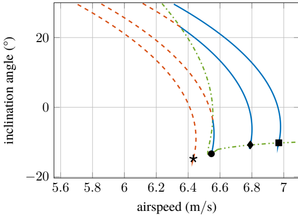
(a) Inclination \gamma over airspeed V_A .
