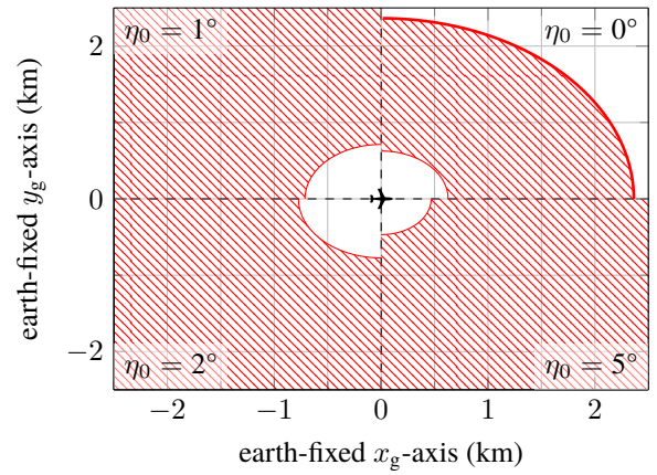
Figure 7: Estimated CFT zones for loss-of-elevator with initial height of 150 m ( ▨ ) and surface positions as indicated.
