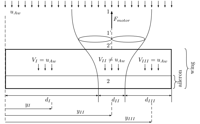
Figure 3: Division of the wing into three sections, with different inflow speeds
