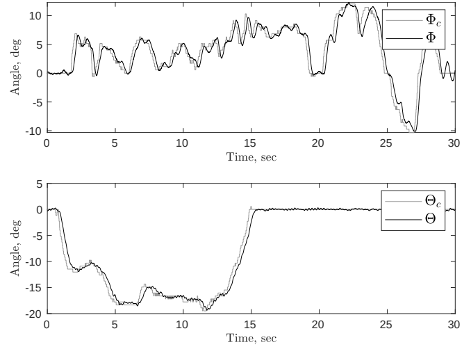
Figure 9: Attitude controller performance in hover flight (experiment)
