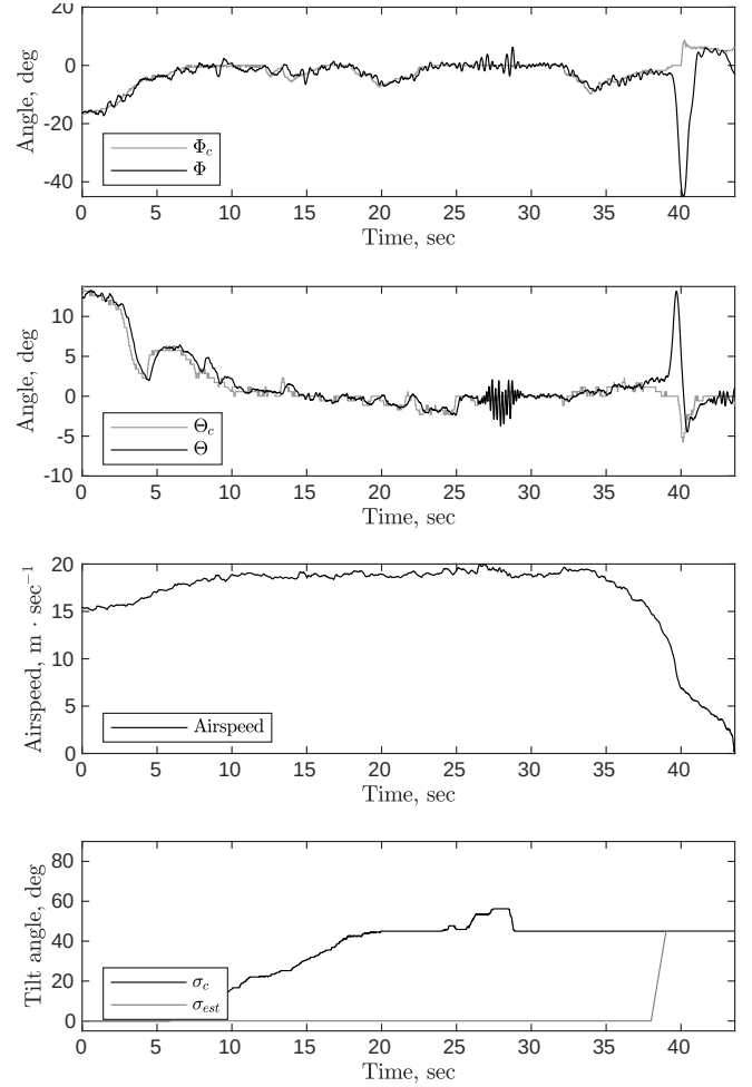
Figure 11: Attitude controller during transition from forward flight to hover (experiment)
