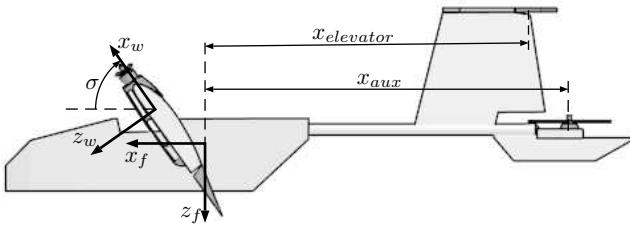
Figure 2: Side view of the aircraft
