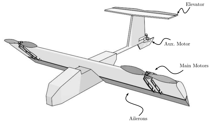
Figure 1: Example tiltwing aircraft in hover configuration
