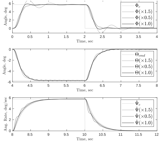
Figure 6: Attitude controller performance in hover flight (simulation)
