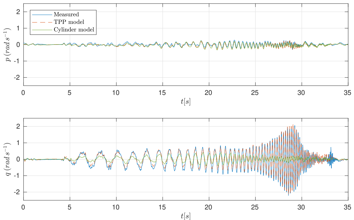
Figure 7: Chirm on the pitch axis in hover. The roll motion due to pitching is much less severe due to the high roll inertia compared to the pitch inertia. Now the CD model's accuracy at low frequencies is also worse than the TPP model.
