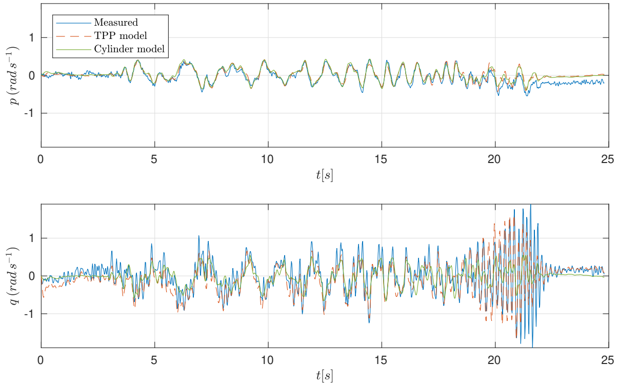
Figure 10: Validation chirp on the elevator axis in forward flight. The roll response q (yaw in standard aircraft reference frame) is fitted accurately by both TPP and CD models, while from around 15 s the CD model is unable to replicate the higher frequencies that the TPP model can still generate. The TPP model is still unable to replicate the highest frequencies of the chirp.
