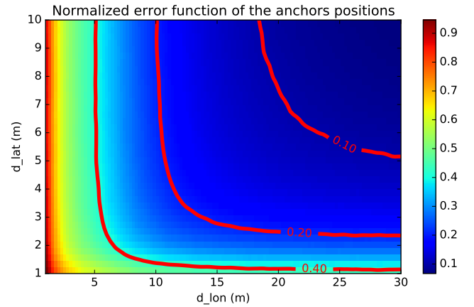
Figure 7: Normalized error score function of d_{lat} and d_{lon} .
