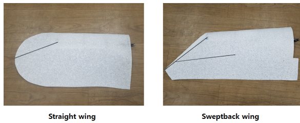
Figure 14: Wing shape
