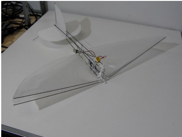
Figure 1 - WiFly
