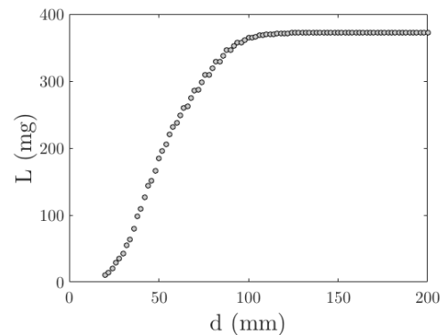
Figure 4: Lift as a function of the characteristic dimension of the control surface.
