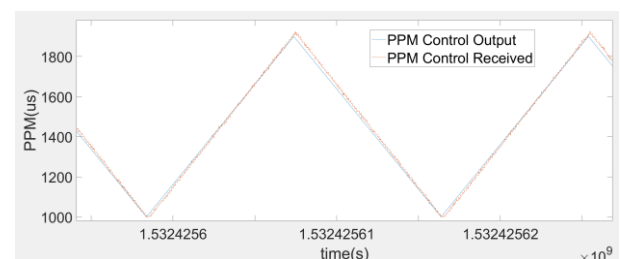
Figure 7-Measured latency
