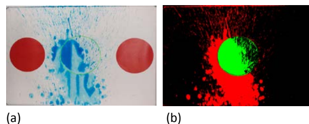
Figure 7 - Spray test sample: (a) raw image (b) image analysed in OpenCV
