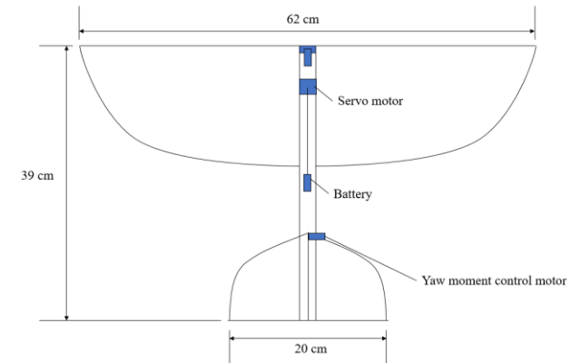
Figure 2 – Dimensional outline of WiFly and components arrangement
