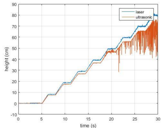
Figure 7 – Altitude estimation
