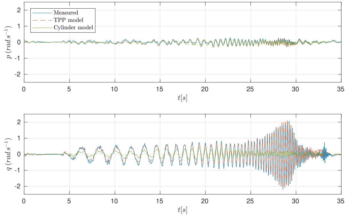
Figure 7: Chirp on the pitch axis in hover. The roll motion due to pitching is much less severe due to the high roll inertia compared to the pitch inertia. Now the CD model's accuracy at low frequencies is also worse than the TPP model.
