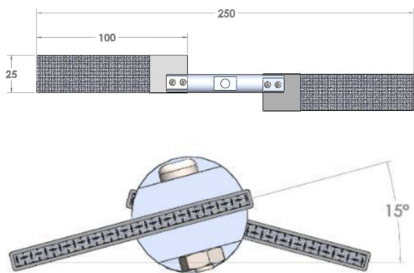
Figure 1 – Rotor geometry
