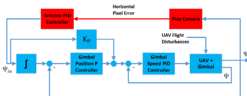
Figure 3 - Target coordinates and control system block diagram for azimuth tracking
