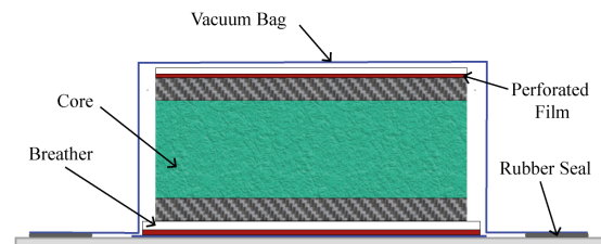
Figure 7: Lay-up technique of the composite frame
