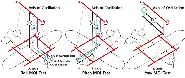
Figure 3: Measurement method of moment of inertia according to flight axis.
