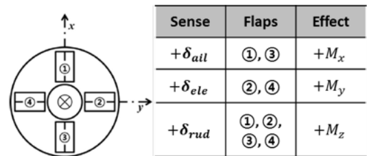
Figure 1: control flaps sign conventions.
