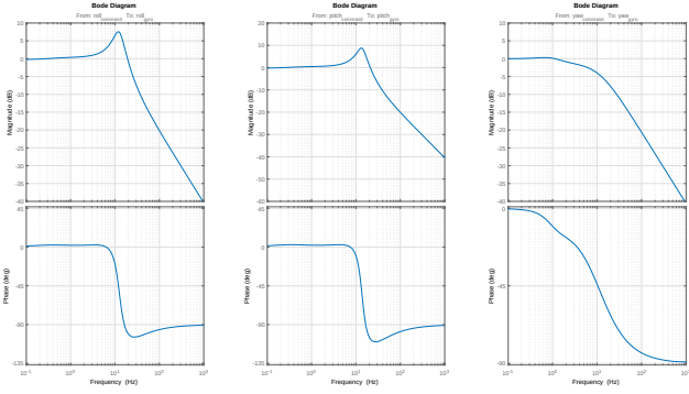
Figure 3: The models generated for the 112mm quadrotor.
