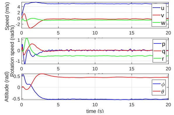
Figure 8: States X
