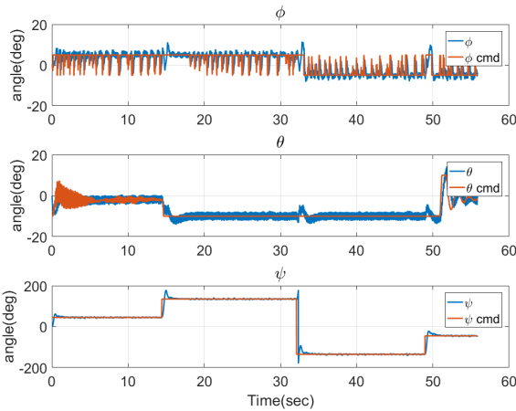
Figure 12: Simulation of disturbance with DOBC
