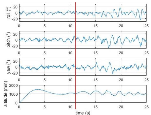
Figure 8 – Attitude and altitude estimation during flight
