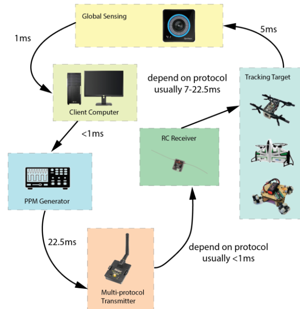
Figure 6 - System latency
