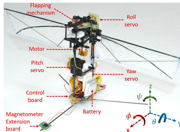
Figure 1 - KUBeetle
