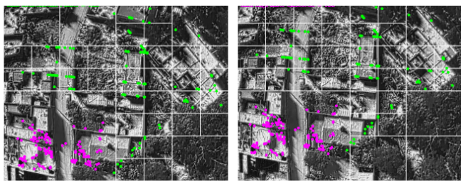
Figure 2: Point correspondences: Green points represent intersection points from inlier line segment correspondences (green lines from Figure 1) and pink points show quadtree-keypoint matches in areas where intersection points were not found.
