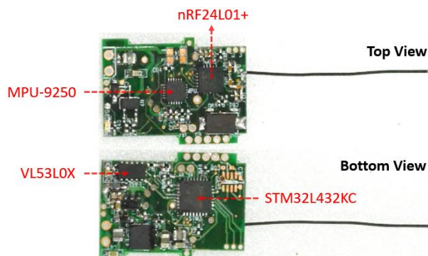
Figure 2 - Control board
