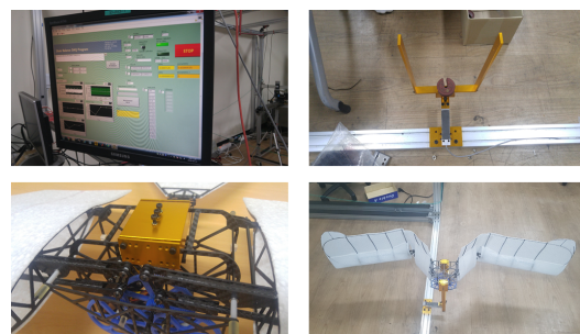
Figure 13: Experiment enviroment
