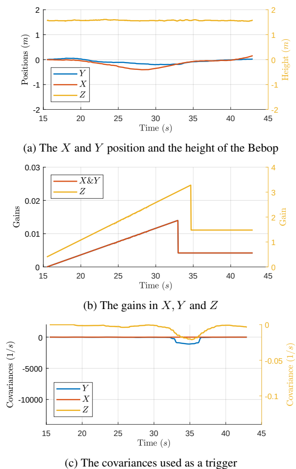
Figure 17: The Bebop with the algorithm applied to the all axes at the same time. A trigger in one horizontal axis will set the gain for both horizontal axes
