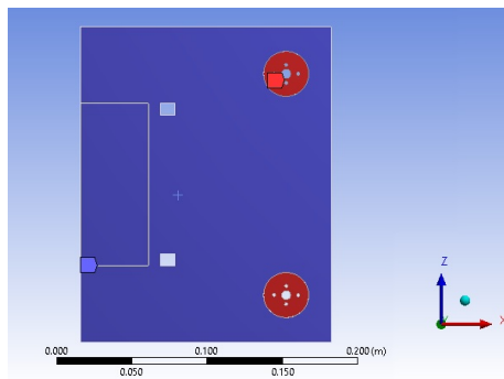
Figure 2: Optimization Region
