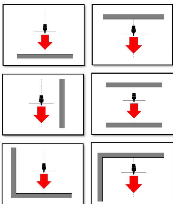
Figure 2 – Wall's configurations
