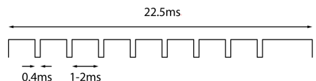
Figure 4 - PPM Signal (8 channels)
