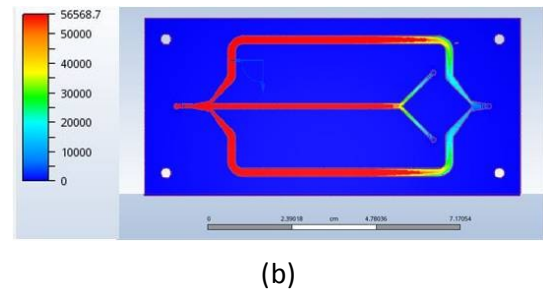
Figure 3 - Flow simulations on the microfluidic chip: Flow division between external and central microchannel (a); flow division between the two tunnels (b). The scale represents the velocity amplitude.
