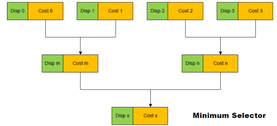
Figure 6: Tree structure comparator for disparity selection
