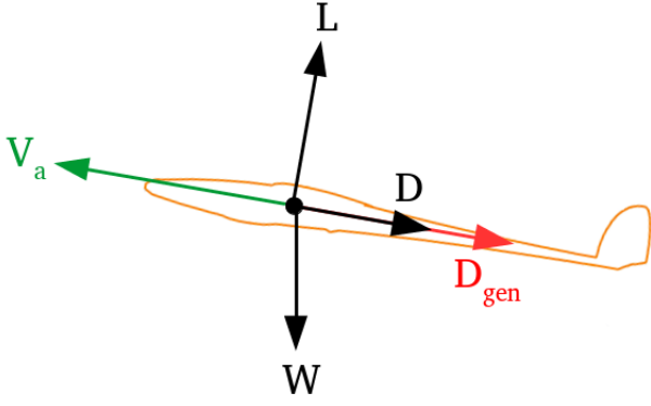
Figure 2: Forces acting on DT-18 UAV developed by Delair (reproduced from Long et al.[12]).
