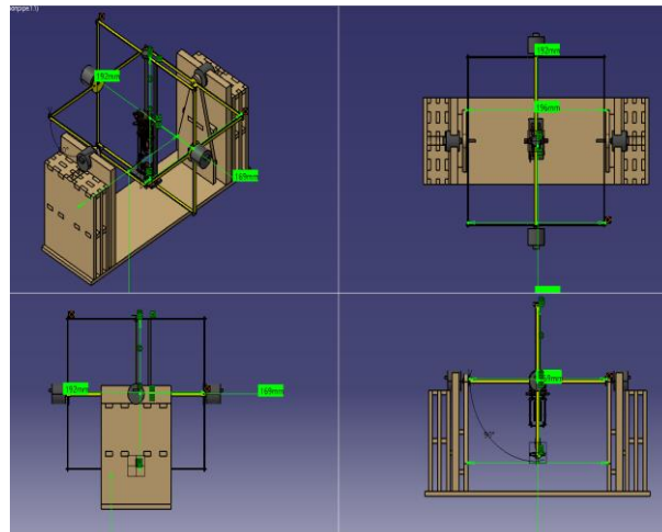
Figure 1 - Conceptual design of 2-DOF rotation measurement verification device for future research
