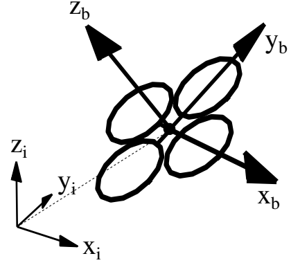
Figure 2 – Aircraft axis system
