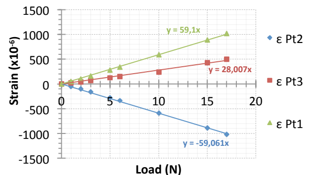
Figure 15 - Experimental wing strain on 3 points
