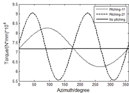
(b) Torque
