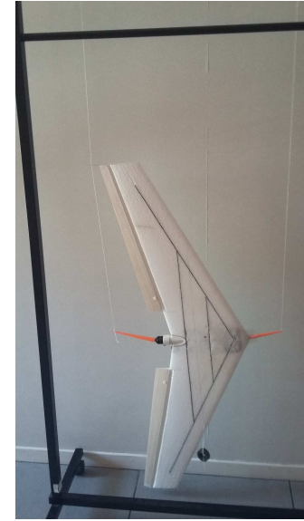
Figure 3: Moment of inertia estimation experiment
