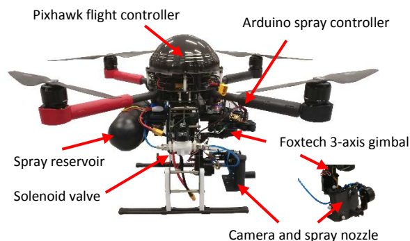
Figure 1 - Multirotor UAV with spray system
