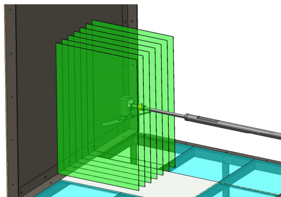
Figure 5 – PIV plane
