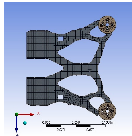
Figure 3: Topology Optimization result
