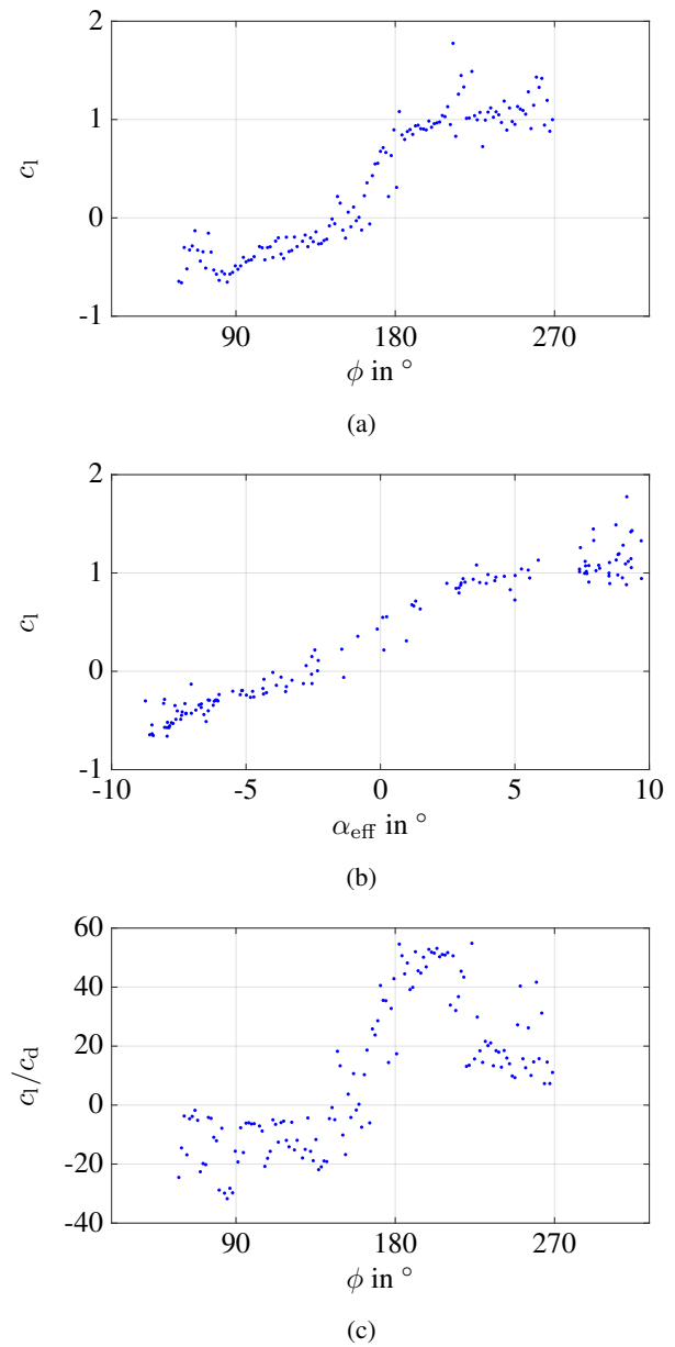
Figure 25: Lift coefficient over phase angle and different effective AOAs as well as lift-to-drag coefficient c_l/c_d over phase angle.
