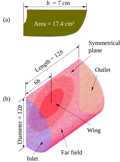
Figure 3 - (a) Wing geometry. (b) Computational domain
