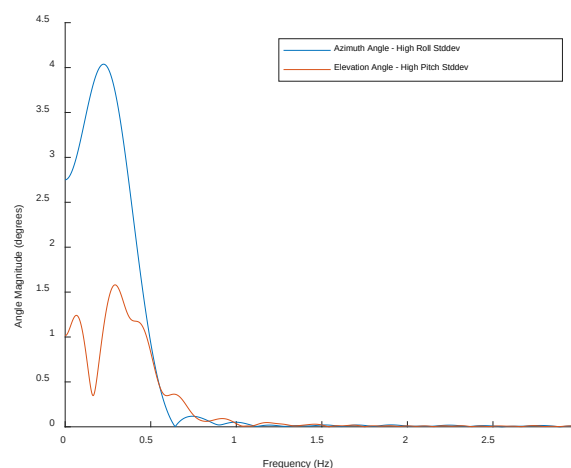
Figure 5 - Frequency spectrum of flight test data
