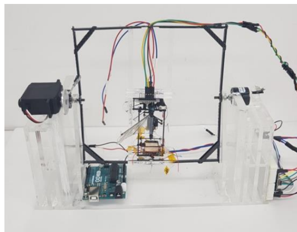
Figure 2 - 1-DOF rotation measurement verification device
