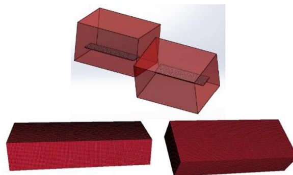
Figure 7 - Blade's Region mesh in CFD simulations
