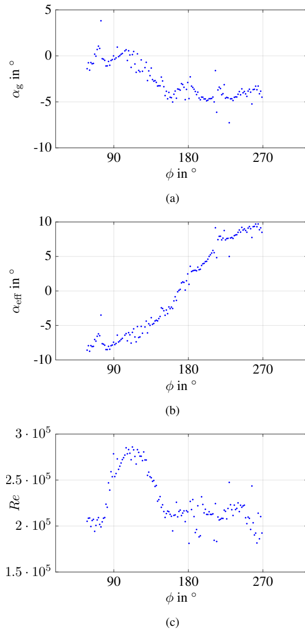
Figure 24: Angle of attack variation \alpha_g and \alpha_{eff} as well as variation of the Reynolds number Re over phase angle.
