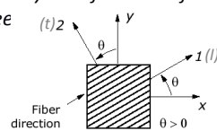
Figure 2 - Fibre orientation
