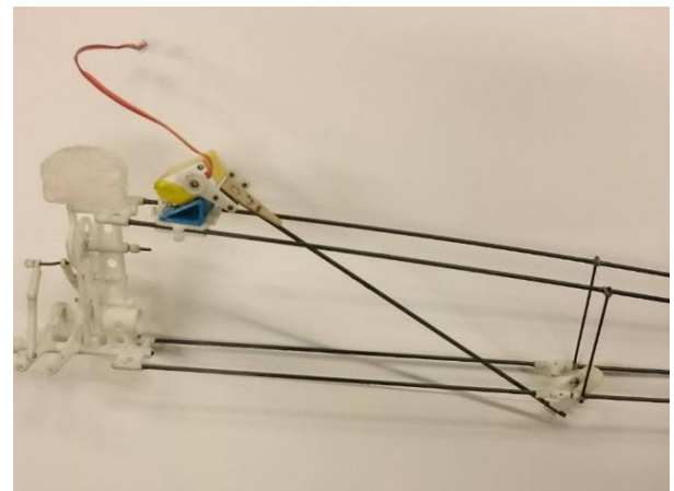
Figure 3 - The COGS mechanism
