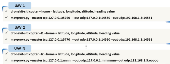
Figure 6: Connect dronekit-sitl and MAVProxy.
