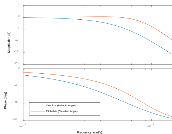
Figure 4 - Bode plot for gimbal yaw and pitch
