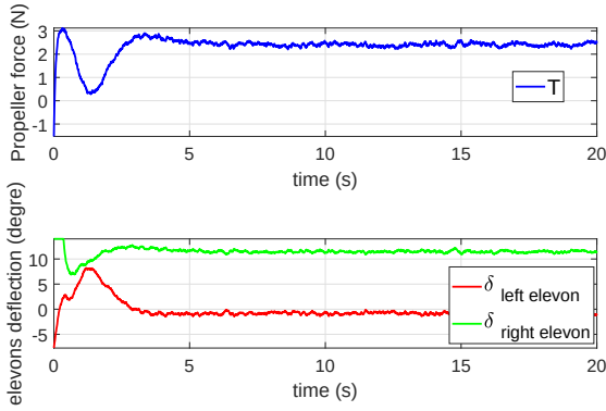
Figure 10: Control U
