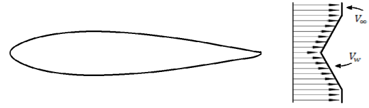
Figure 2: Airfoil and velocity distribution of the wake.
