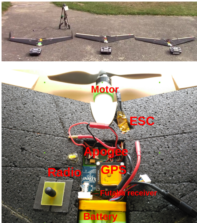
Figure 4: The three custom flying-wings employed for the formation flight parade equipped with Paparazzi autopilot.
