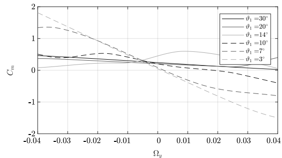
Figure 8: Longitudinal static stability analysis regarding the slope of the pitching moment coefficient C_m with respect to the dimensionless pitch rate \Omega_y = q \cdot c / V^A for different tilt angles \vartheta_1 in trimmed steady horizontal flight.
