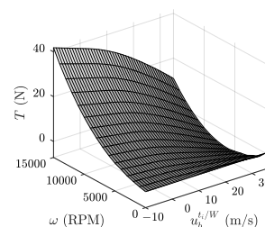
Figure 3: Propeller thrust.
