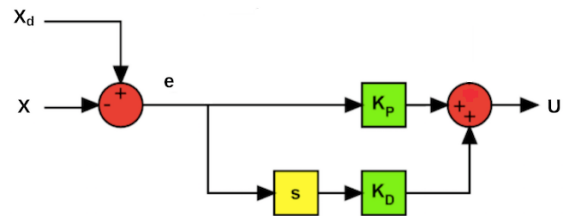
Figure 3: PD Controller Diagram
