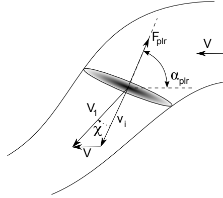
Figure 3: A propeller in oblique flow.
