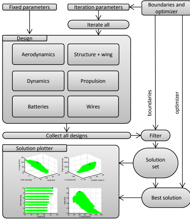
Figure 6: Overview of the design algorithm.
