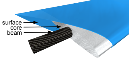
Figure 2: Lightweight construction of a UAV wing.
