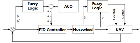
Figure 7: Deviation correction and stability augmentation control system
