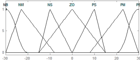
Figure 4: Membership function of elevator deflection
