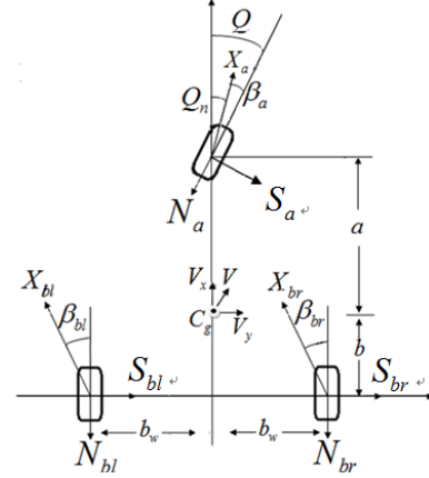
Figure 1: Ground force acting on tires
