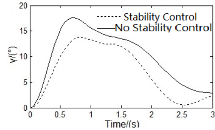
Figure. 8: Change of roll angle during deviation correction
