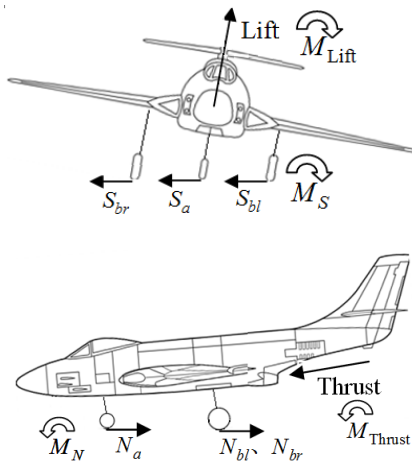
Figure 2: Analysis of rollover force
