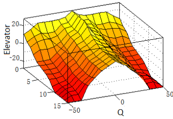
Figure 5: Fuzzy control rules of elevator
