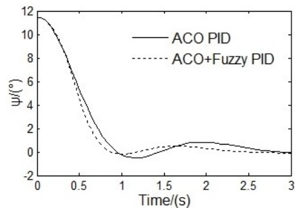
Figure 10: Change of yaw angle during deviation correction
