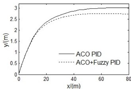
Figure 11: Taxiing track during deviation correction
