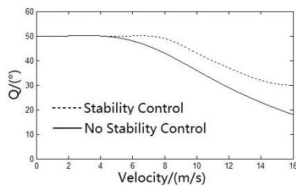
Figure 9: Critical condition of taxiing rollover
