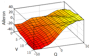
Figure 6: Fuzzy control rules of aileron
