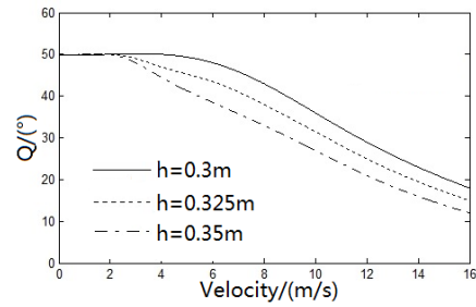
Figure 3: Critical condition of taxiing rollover
