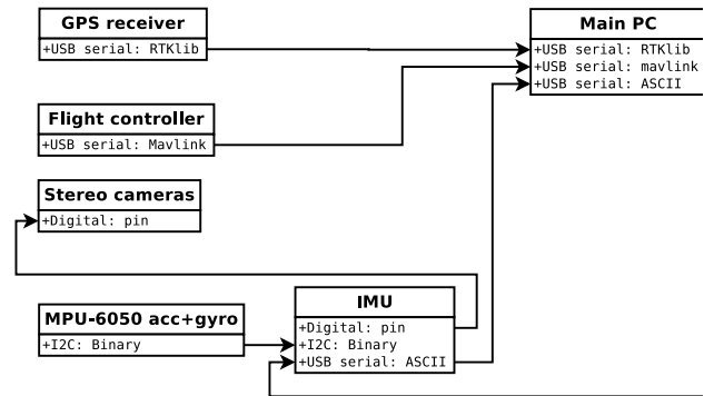
Figure 3: A schematic of the onboard hardware and their connections.
