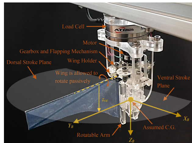
Figure 7: Experimental setup.
