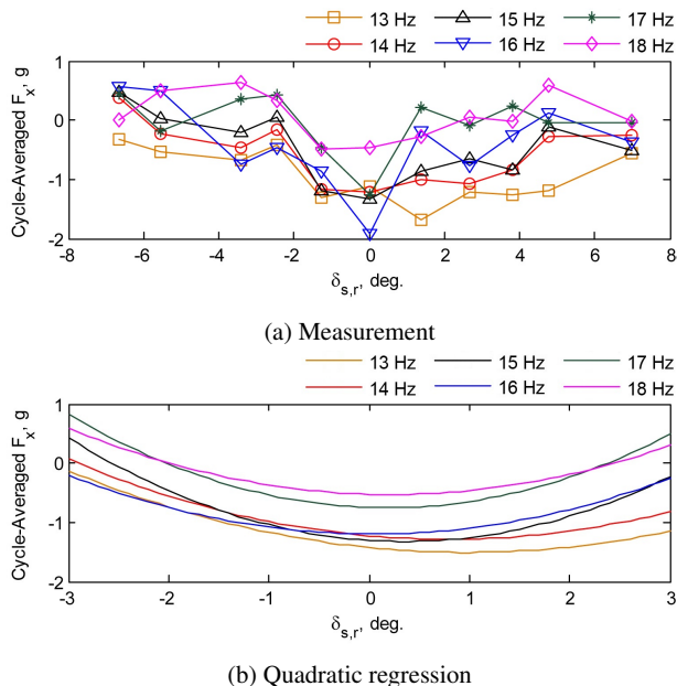
Figure 11: Cycle-averaged forward force.
