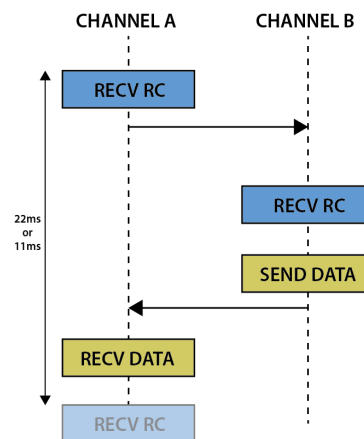
Figure 7: SuperbitRF protocol
