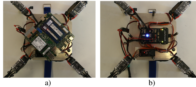
Figure 3: Image conversions
