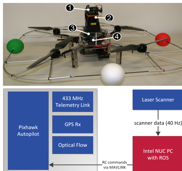
Figure 1: Quadrotor UAS
