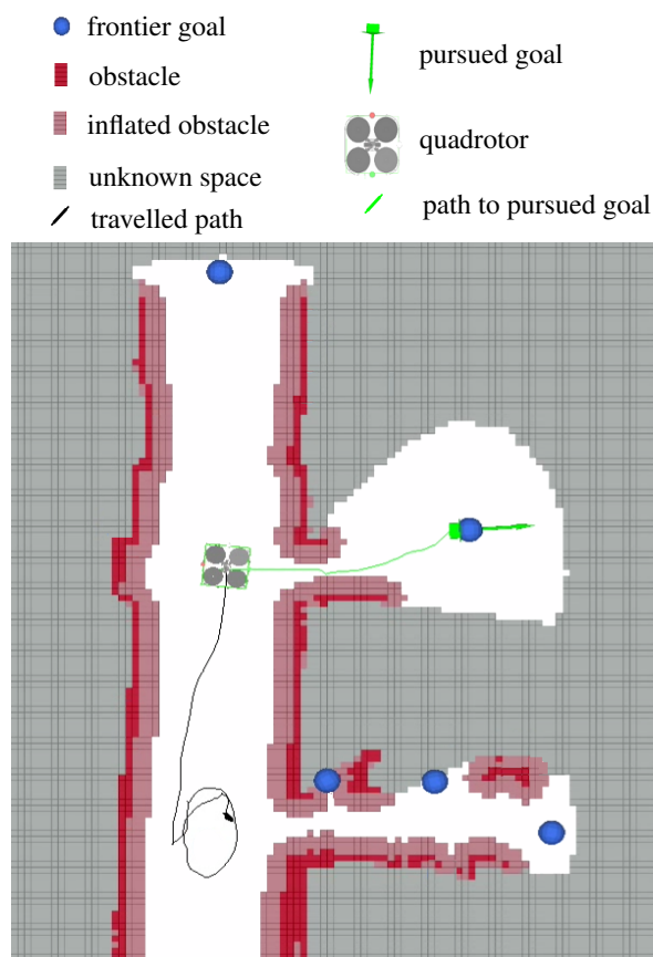
Figure 7: Exploration algorithm
