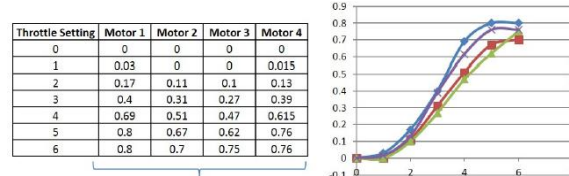
Fig. 21 Motor Thrust Indifferences graph and Table
