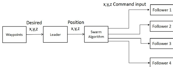
Fig. 24 Block representation of Leader Follower Method
