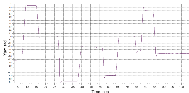
Figure 7: Measured yaw angle
