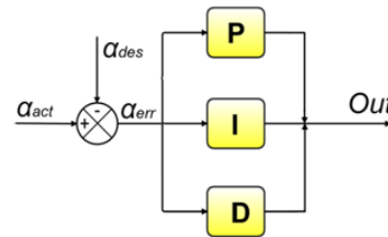
Figure 8: PID control block diagram
