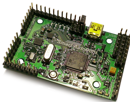
Figure 2: SmartAP v2.0 Hardware
