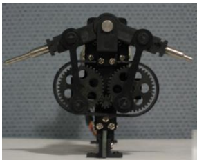
Fig. 3 (left): Dual Gear Crank
