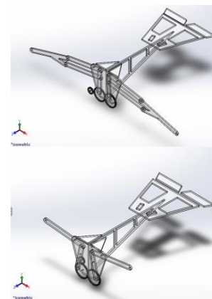
Fig. 8 (left): Articulated Flapping Wing
